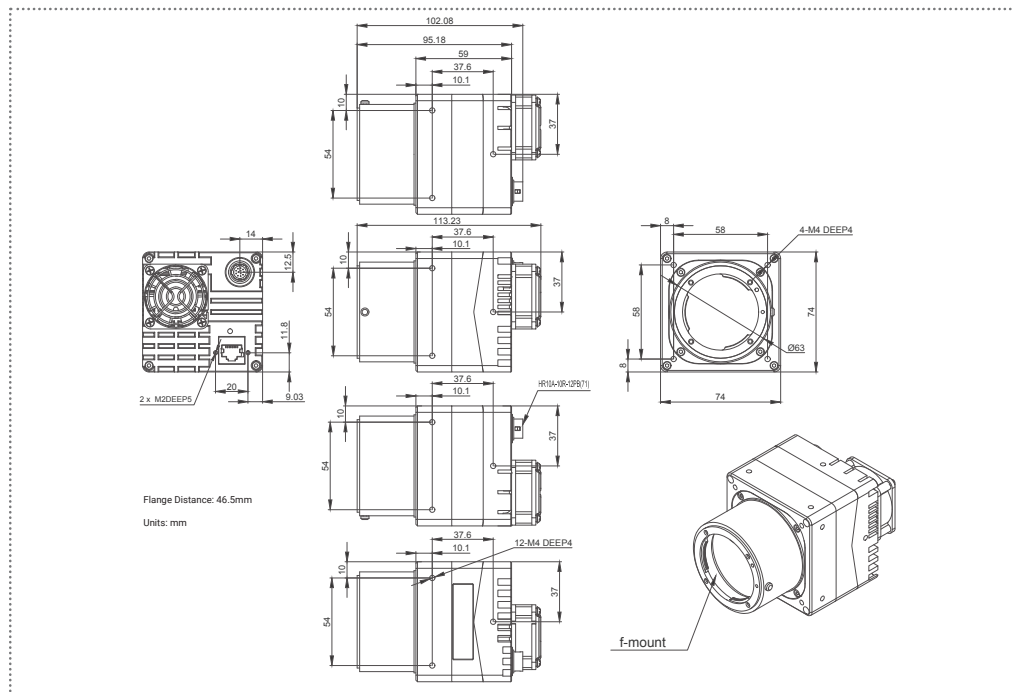
MARS-5000-24GTM/C-NF F, F-mount
