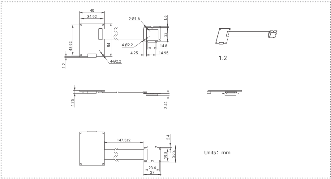
VEN-302-56U3M/C-S, No-mount
