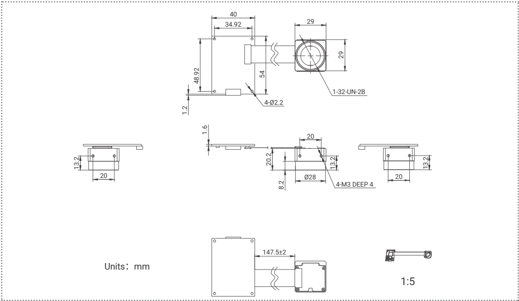
VEN-302-56U3M/C-S, C-mount
