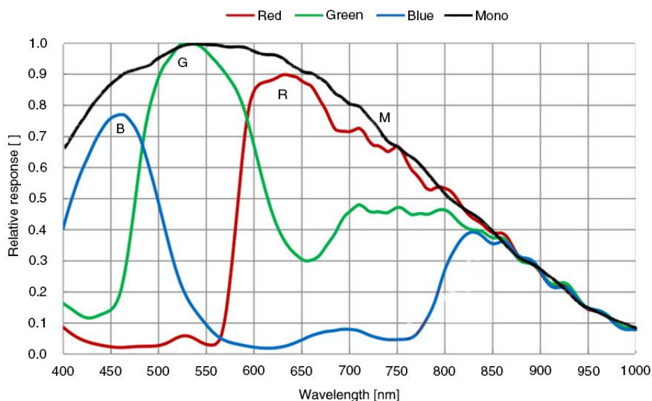
Figure 4-36 ME2S-2440-16U3M/C sensor spectral response
