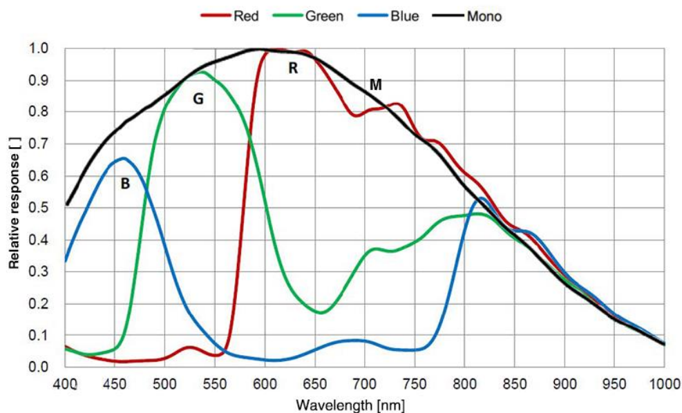
Figure 4-16 MER2-502-79U3M/C(-L) sensor spectral response
