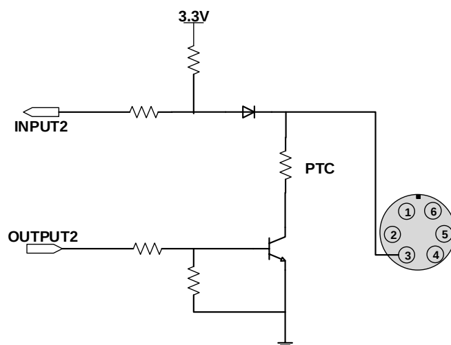
Figure 7-13 Line2 (bidirectional) circuit (MER2-6P/ME2S)
