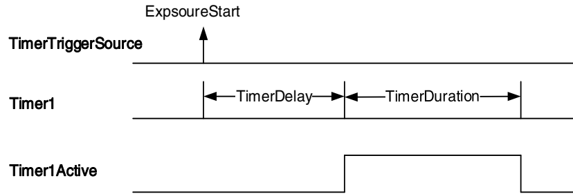
Figure 8-66 Timer1Active schematic diagram
