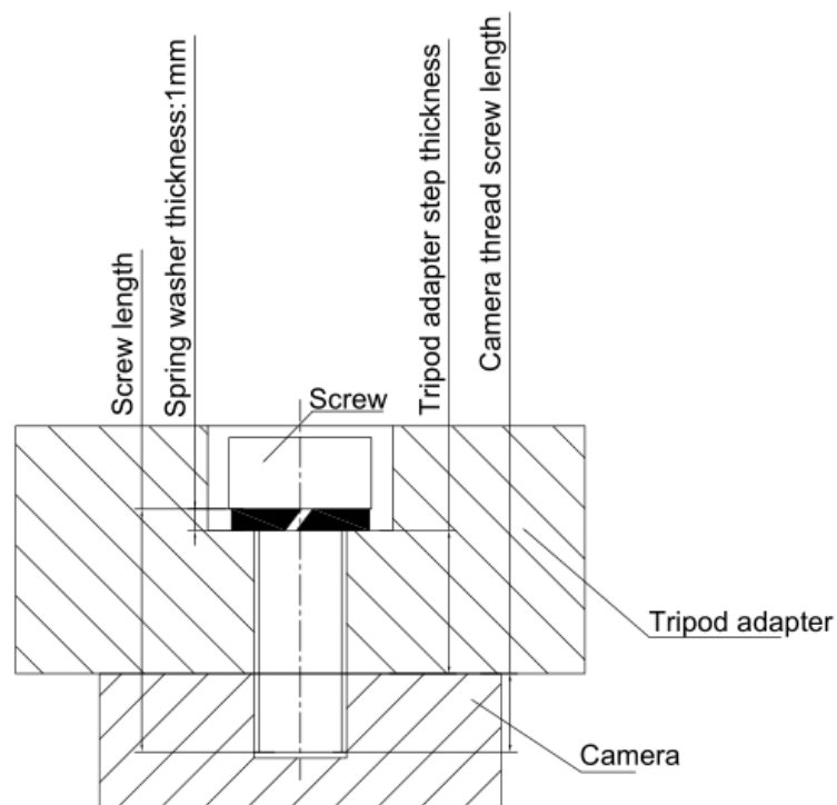
Figure 5-15 Schematic diagram of screw specification, tripod adapter step thickness and spring washer thickness
