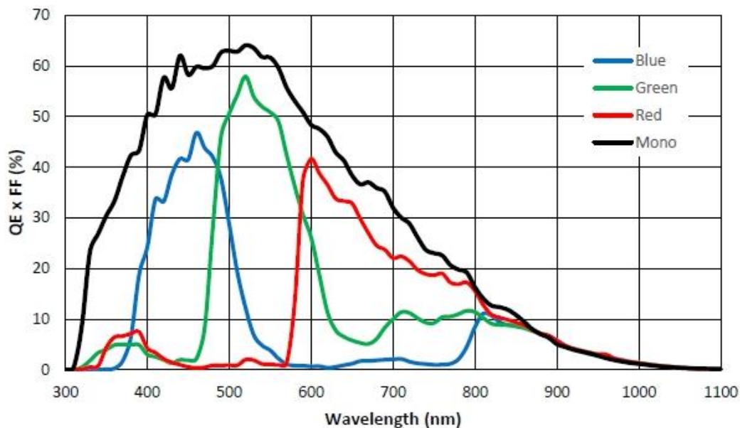
Figure 4-49 ME2P-1840-21U3M/C sensor spectral response
