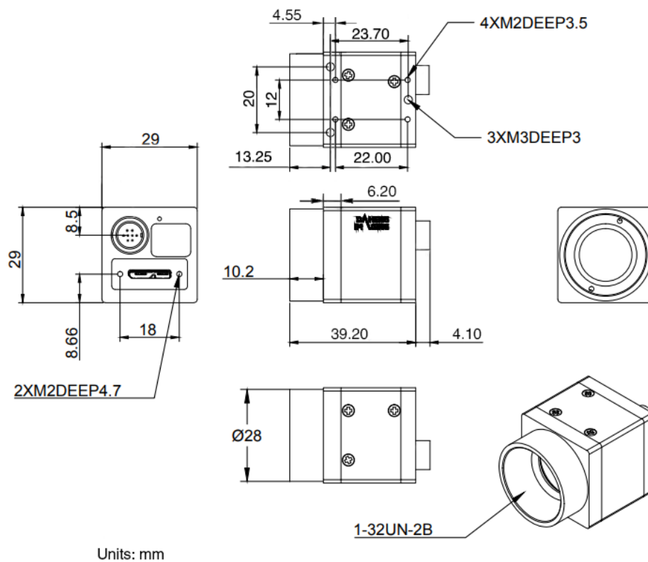
Figure 5-10 ME2L-U3 mechanical dimensions
