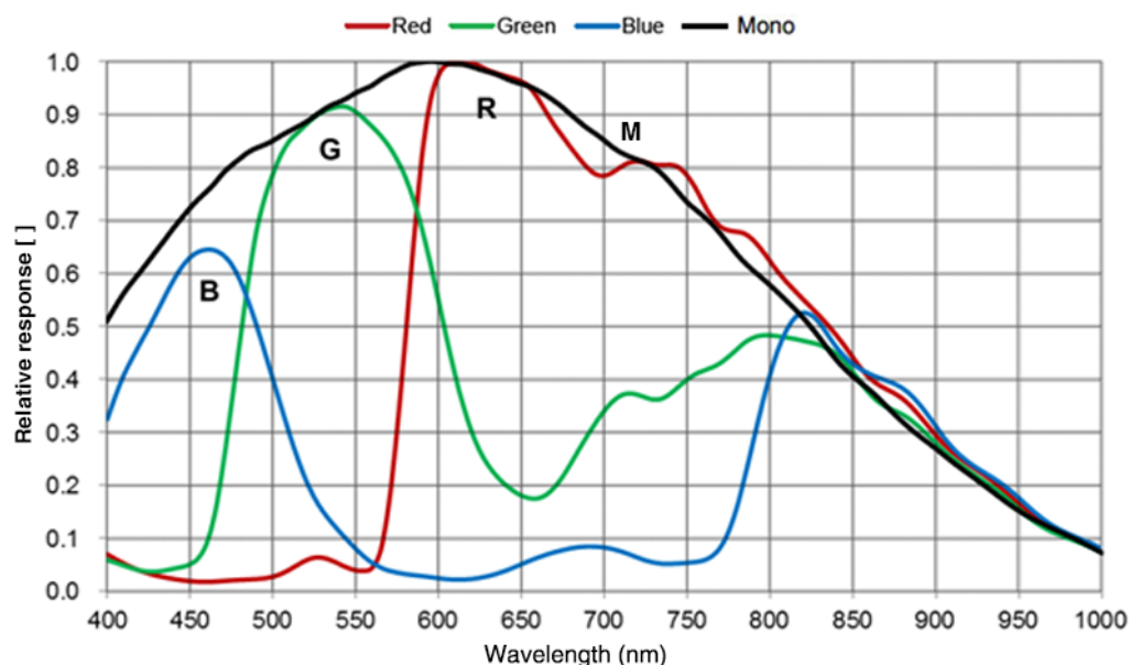
Figure 4-47 ME2P-1231-32U3M/C sensor spectral response
