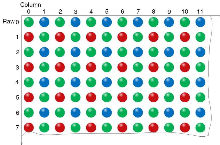
Figure 8-41 BayerGB8 pixel format
