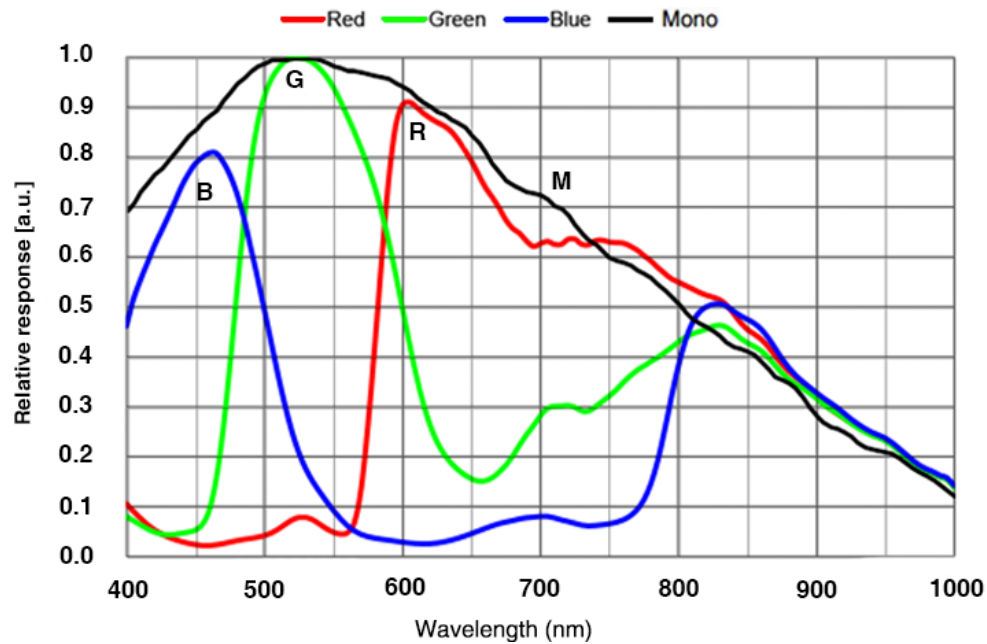
Figure 4-58 ME2L-505-36U3M/C(-L) sensor spectral response
