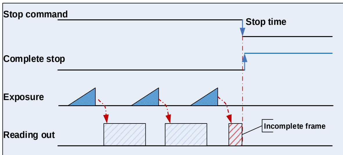
Figure 8-17 Acquisition stop during reading out
