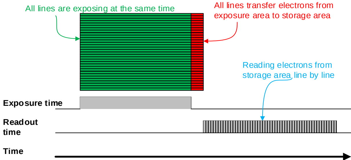
Figure 8-32 Global shutter
