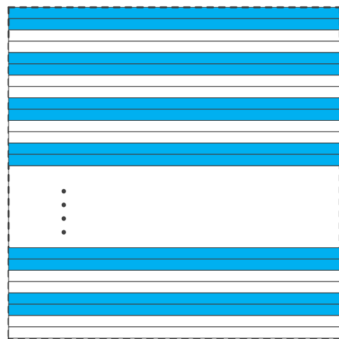
Figure 8-53 Color camera vertical Decimation
