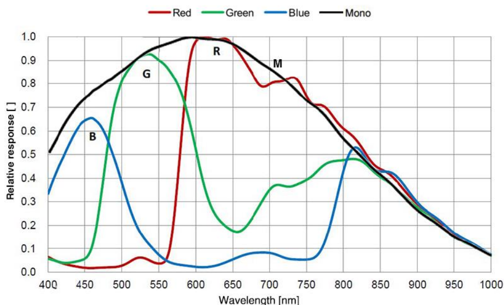
Figure 4-27 MER2-301-125U3M/C(-L)-HS sensor spectral response
