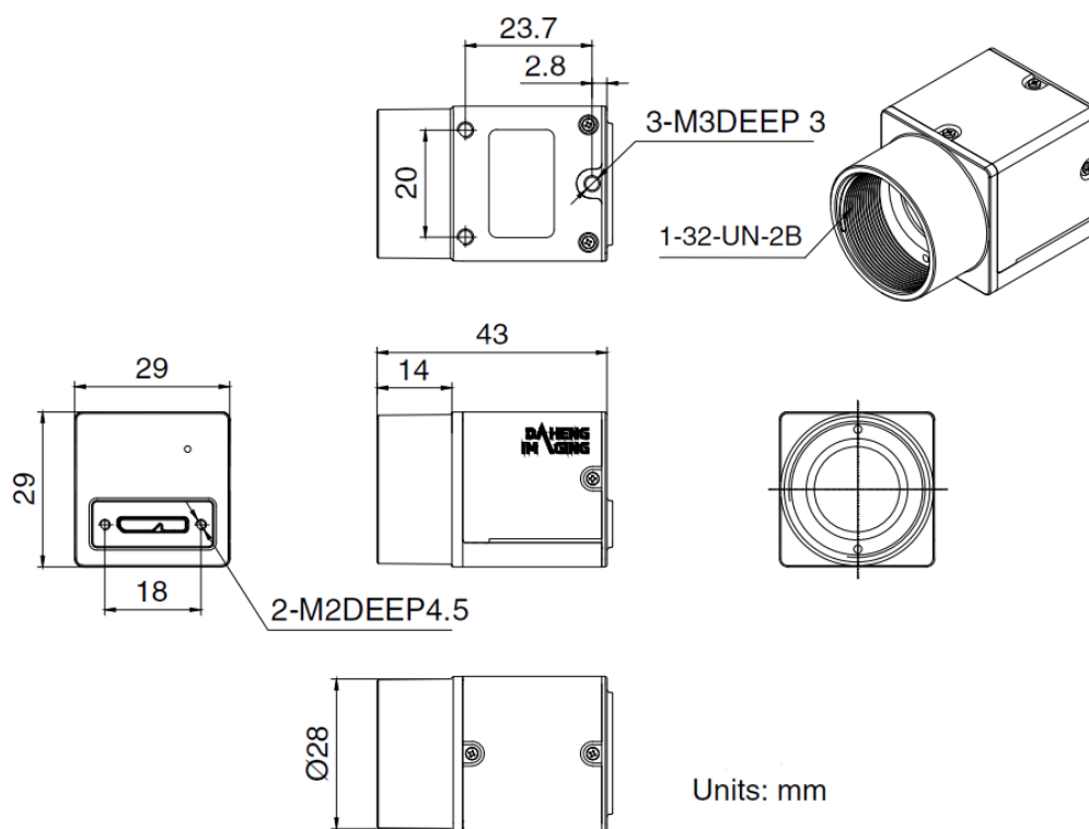
Figure 5-6 MER2-U3-L-6P mechanical dimensions
