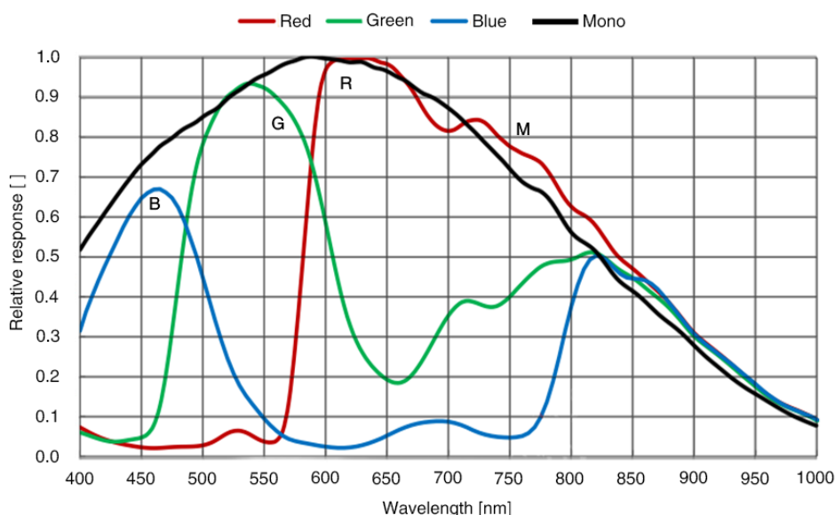
Figure 4-10 MER2-280-139U3M/C(-L) sensor spectral response
