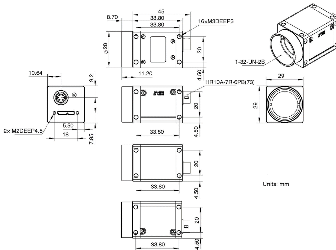
Figure 5-7 ME2S-U3 mechanical dimensions
