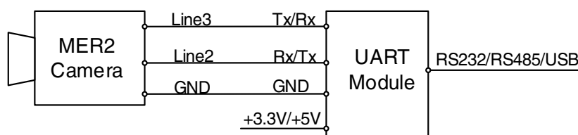
Figure 8-101 The wiring diagram of the camera and external serial port device
