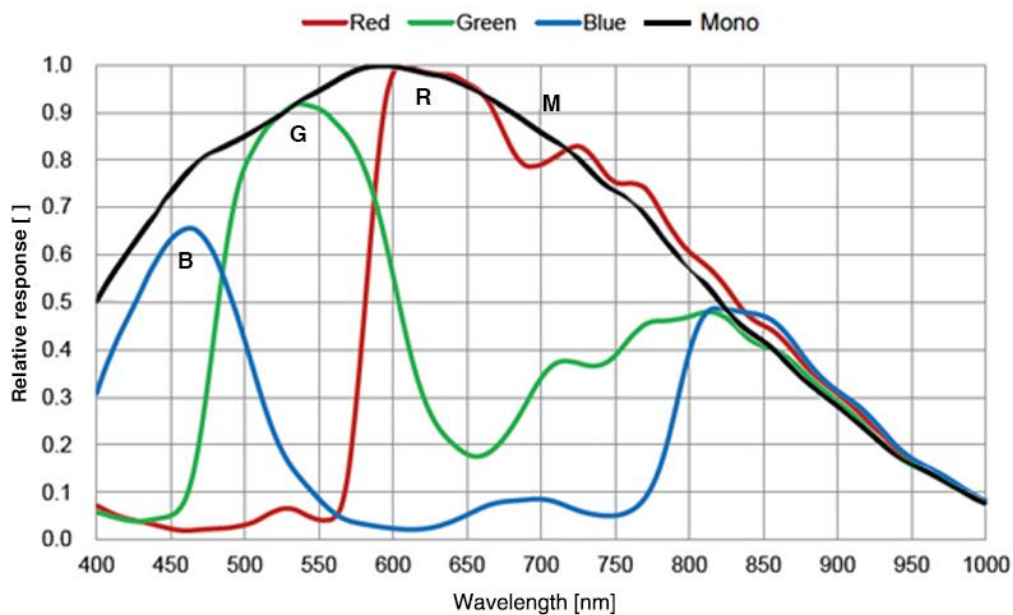
Figure 4-31 MER2-160-249U3M/C(-L)-HS-6P sensor spectral response
