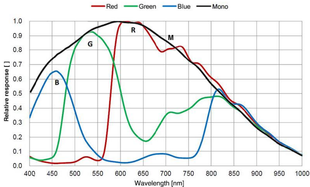
Figure 4-11 MER2-301-125U3M/C(-L) sensor spectral response
