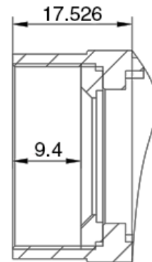
Figure 5-13 C-mount optical interface of ME2L
