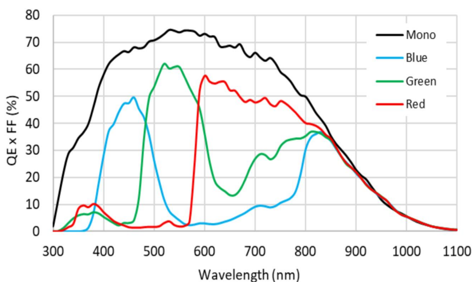
Figure 4-9 MER2-240-159U3M/C(-L) sensor spectral response
