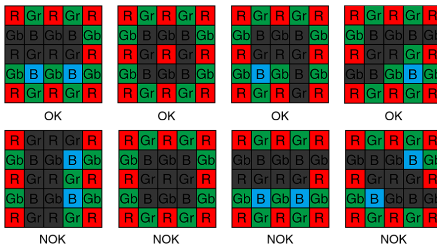
Figure 4-53 ME2P-2622-15U3C clusters within different Bayer color plane distribution diagram
