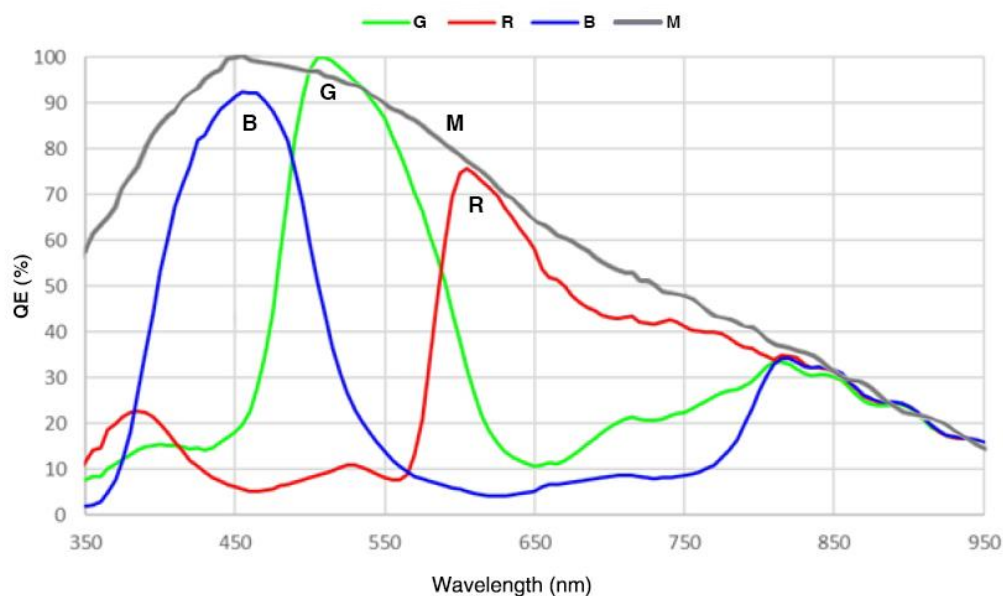
Figure 4-4 MER2-135-150U3M/C(-L) sensor spectral response
