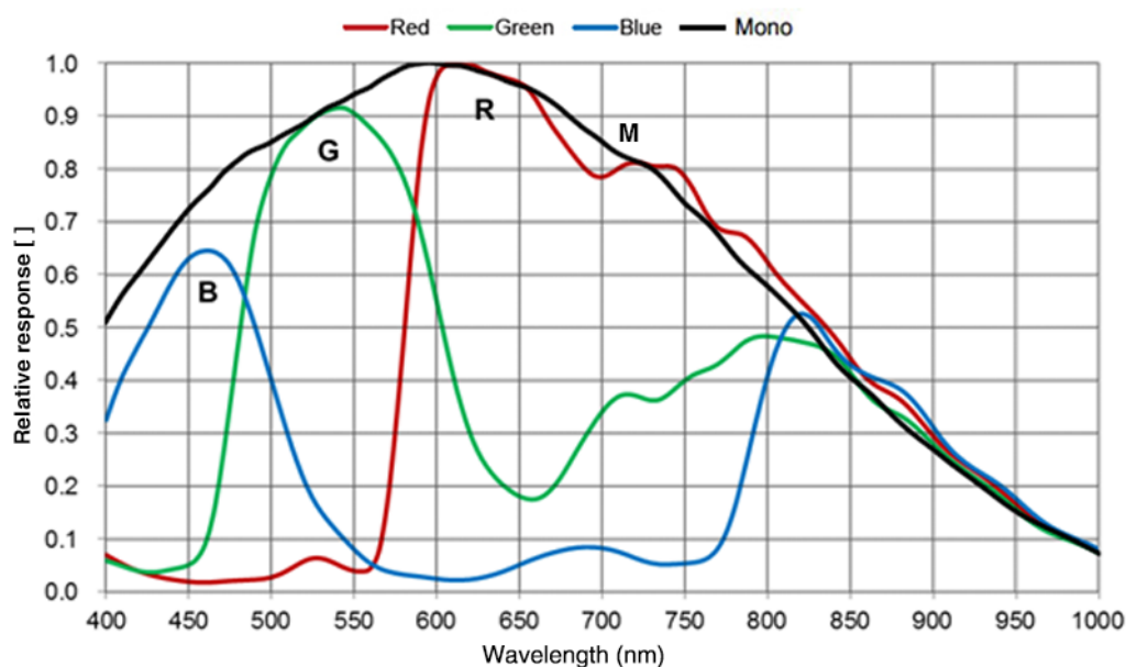
Figure 4-46 ME2P-1230-23U3M/C sensor spectral response
