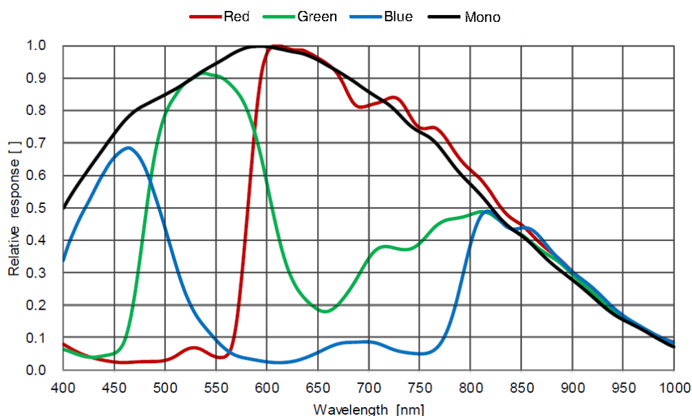
Figure 4-56 ME2L-042-121U3M/C(-L) sensor spectral response
