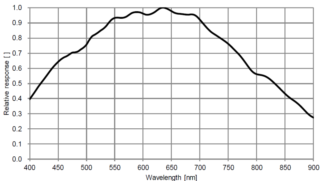
Figure 4-48 ME2P-1231-32U3M POL sensor spectral response
