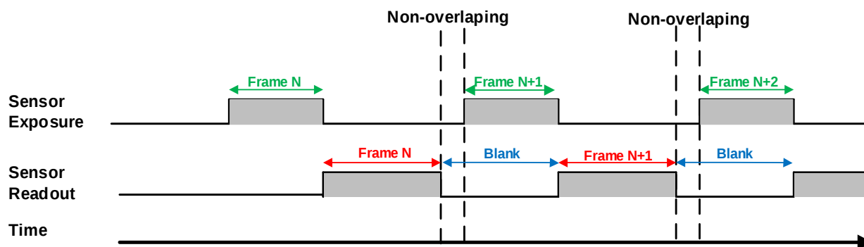
Figure 8-24 The exposure sequence diagram in non-overlapping exposure mode
