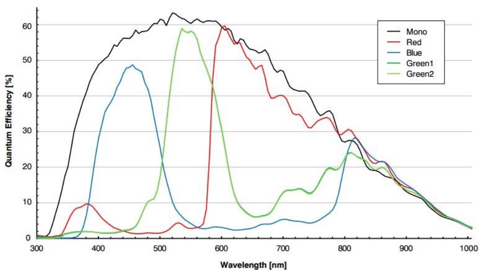
Figure 4-33 ME2S-1260-28U3M/C sensor spectral response
