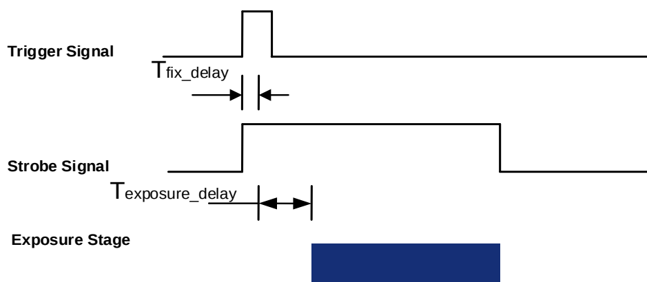
Figure 8-35 The exposure delay sequence diagram in overlapping exposure mode
