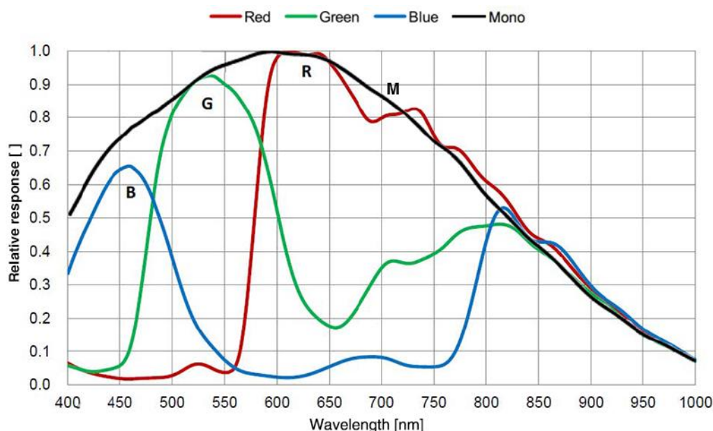
Figure 4-18 MER2-503-36U3M/C(-L) sensor spectral response
