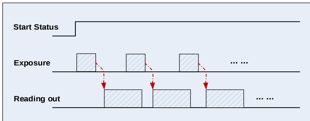
Figure 8-15 Continuous acquisition process
