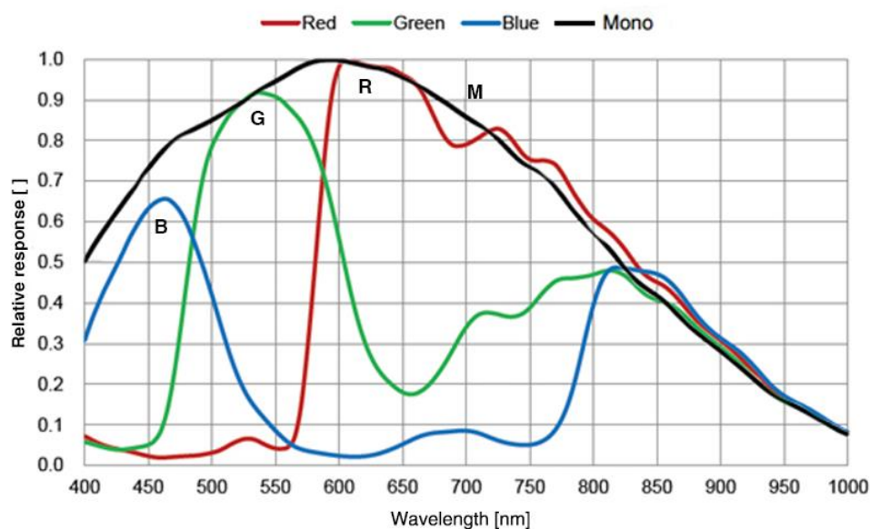
Figure 4-6 MER2-160-227U3M/C(-L) sensor spectral response
