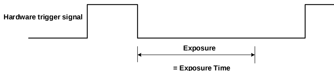
Figure 8-29 The sequence diagram in falling edge trigger of Timed exposure mode
