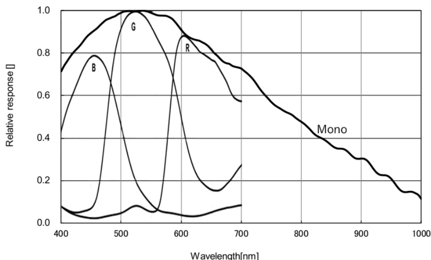
Figure 4-22 MER2-1220-32U3M/C(-L/-W90/-W90-S90) sensor spectral response
