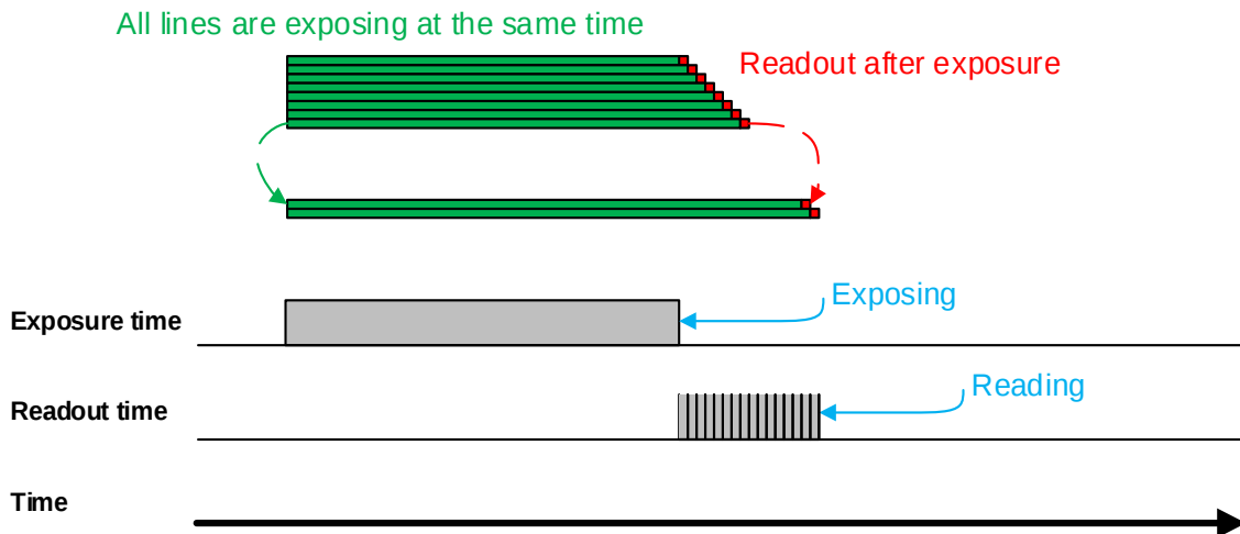
Figure 8-34 Global Reset Release shutter
