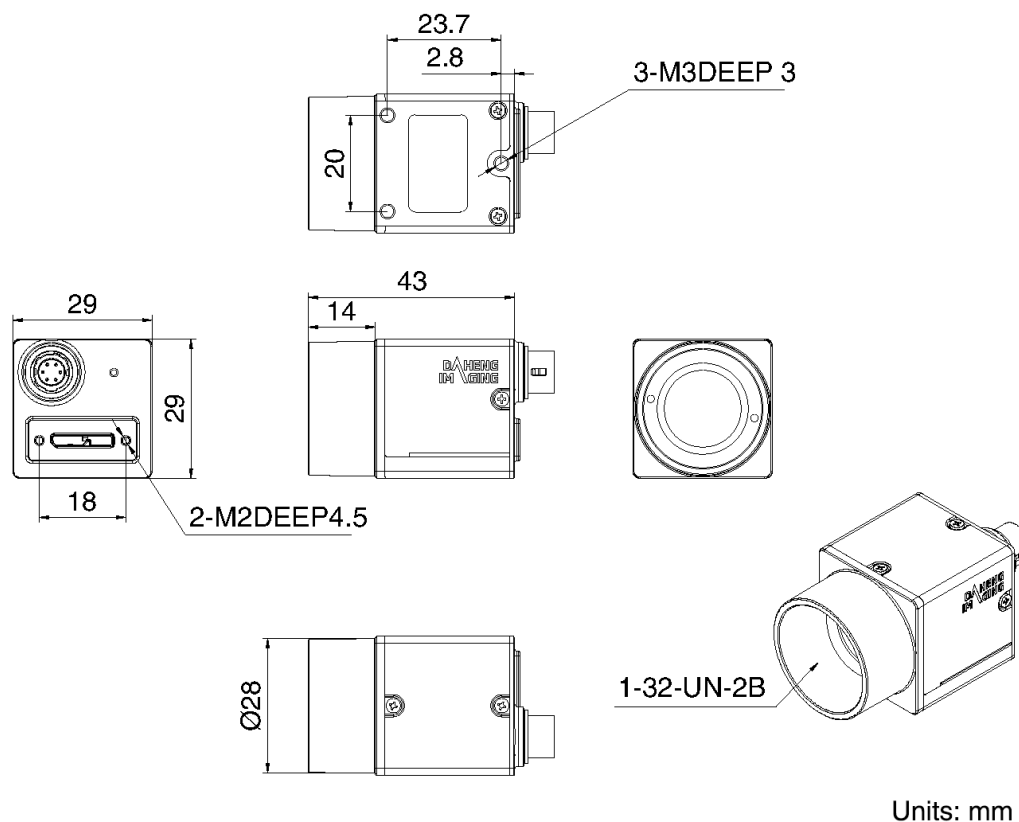
Figure 5-5 MER2-U3-6P mechanical dimensions
