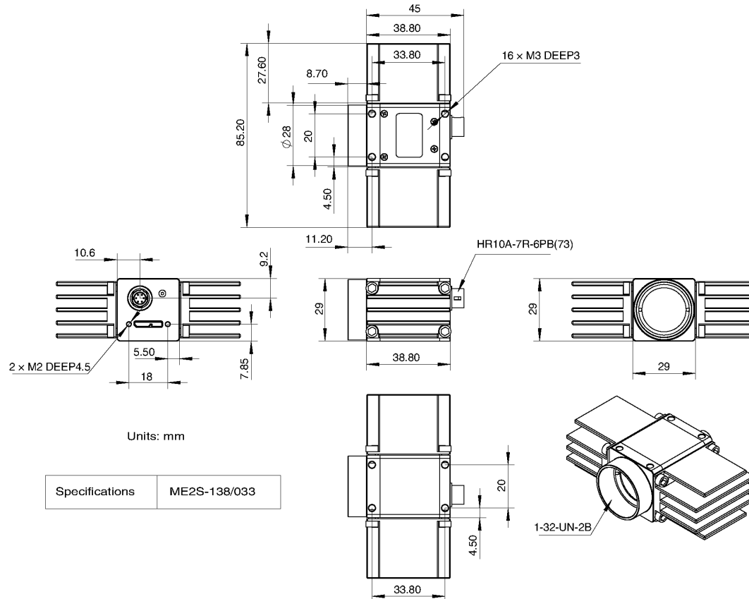
Figure 5-8 ME2S-U3 mechanical dimensions (With Heat Dissipation Fins)
