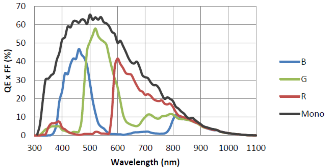
Figure 4-43 ME2P-560-36U3M/C sensor spectral response
