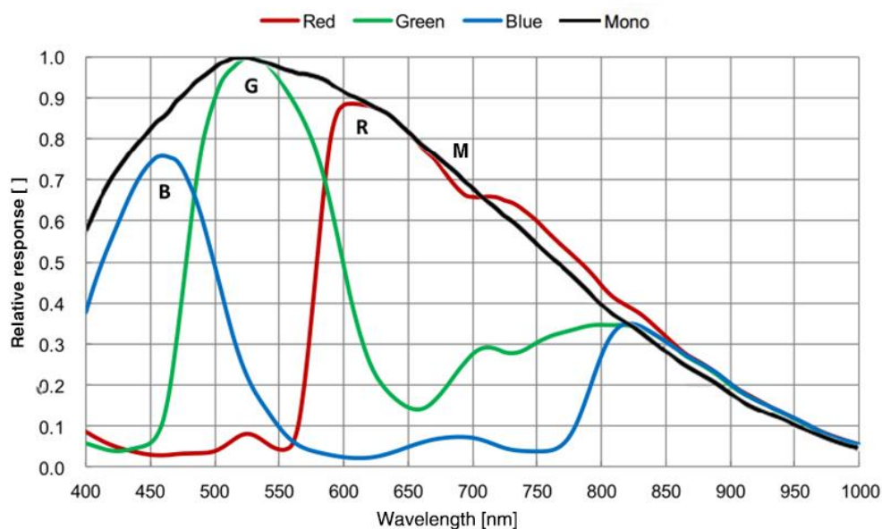
Figure 4-7 MER2-230-168U3M/C(-L) sensor spectral response
