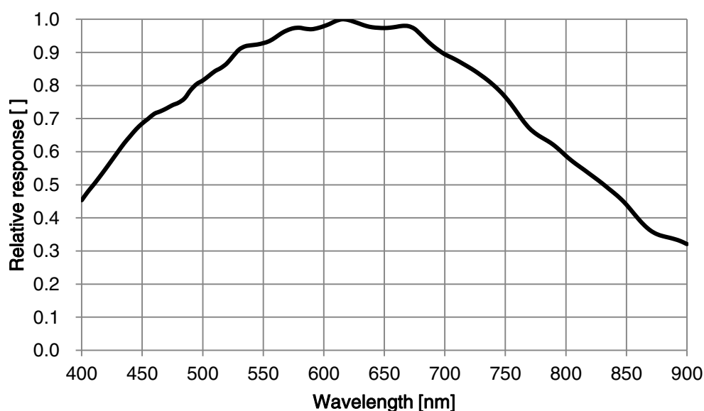
Figure 4-17 MER2-502-79U3M POL sensor spectral response
