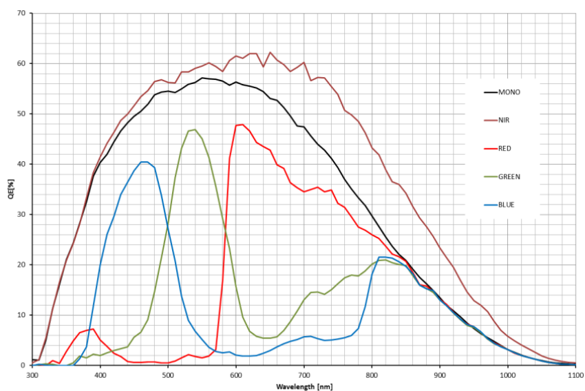
Figure 4-42 ME2P-530-72U3M NIR \ ME2P-530-72U3C sensor spectral response
