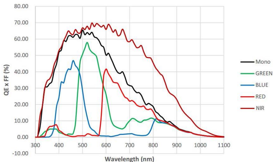
Figure 4-54 ME2P-2621-15U3M NIR \ ME2P-2622-15U3M NIR sensor spectral response
