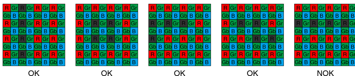
Figure 4-52 ME2P-2622-15U3C clusters within same Bayer color plane distribution diagram
