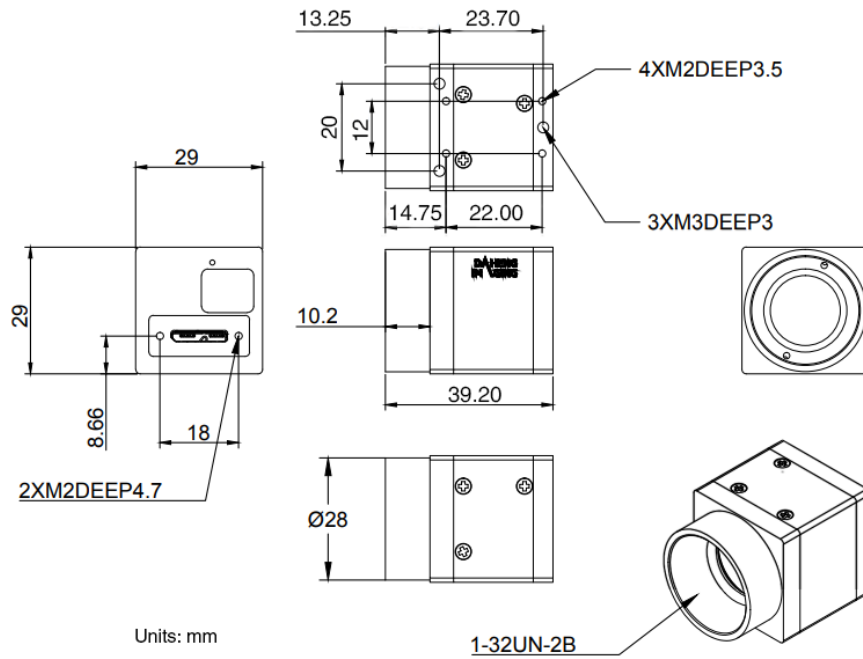
Figure 5-11 ME2L-U3-L mechanical dimensions
