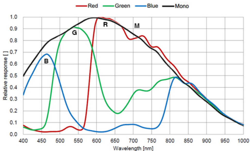
Figure 4-30 MER2-041-608U3M/C(-L)-HS-6P sensor spectral response
