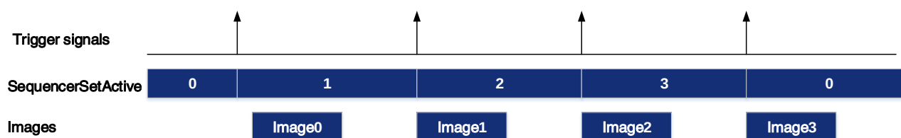
Figure 8-103 Timing diagram
