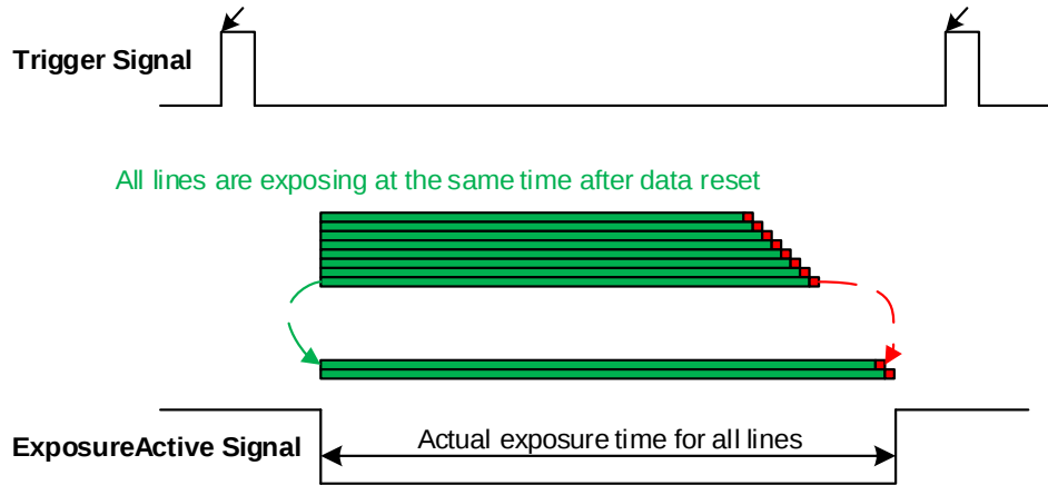
Figure 8-10 Global reset release shutter mode "ExposureActive" signal schematic diagram
