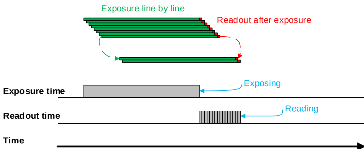
Figure 8-33 Electronic rolling shutter
