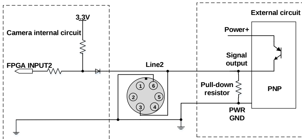
Figure 7-22 PNP photoelectric sensor connected to Line2 input circuit (MER2-6P/ME2S)
