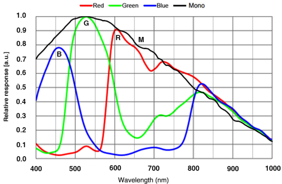
Figure 4-59 ME2L-830-22U3M/C(-L) sensor spectral response
