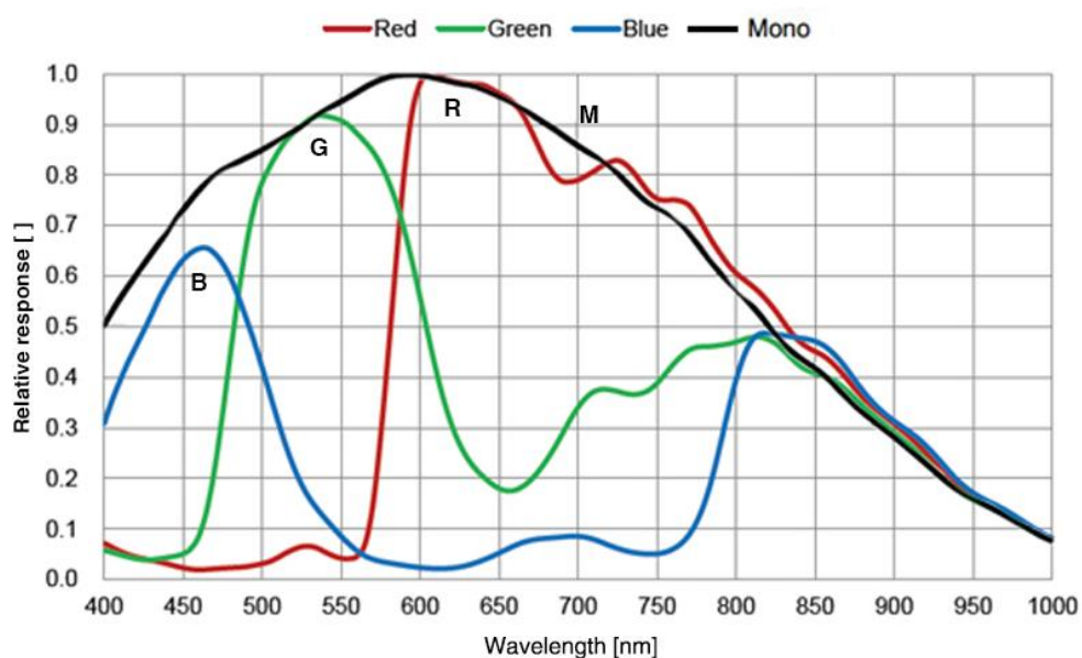
Figure 4-57 ME2L-161-61U3M/C(-L) sensor spectral response
