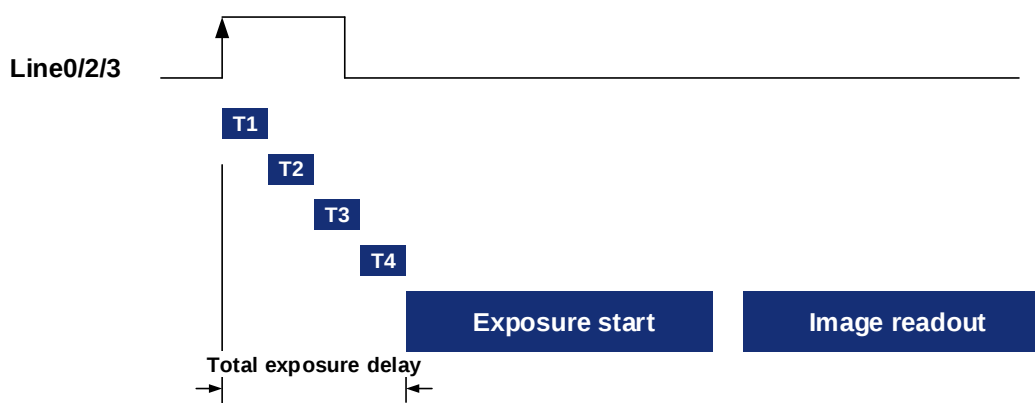
Figure 8-36 Exposure delay
