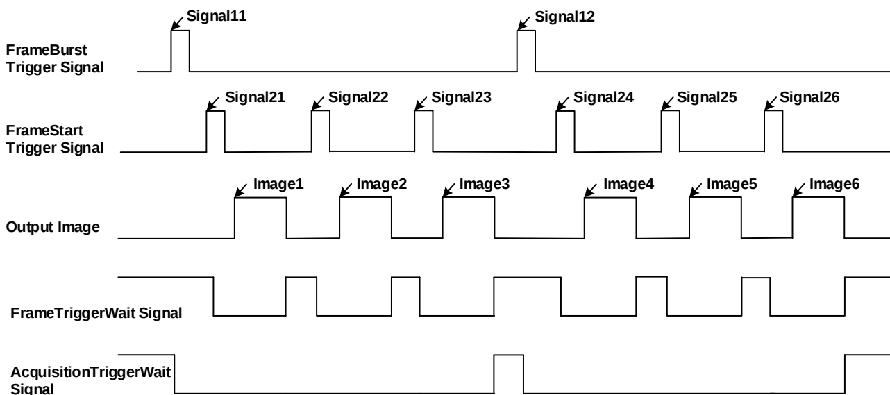
Figure 8-13 "TriggerWait" signal schematic diagram when "FrameBurstStart" and "FrameStart" enabled simultaneously
