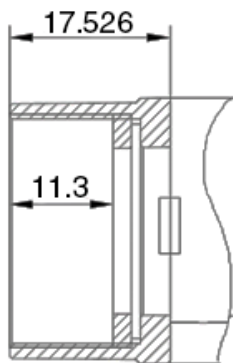
Figure 5-12 C-mount optical interface of ME2P/MER2
