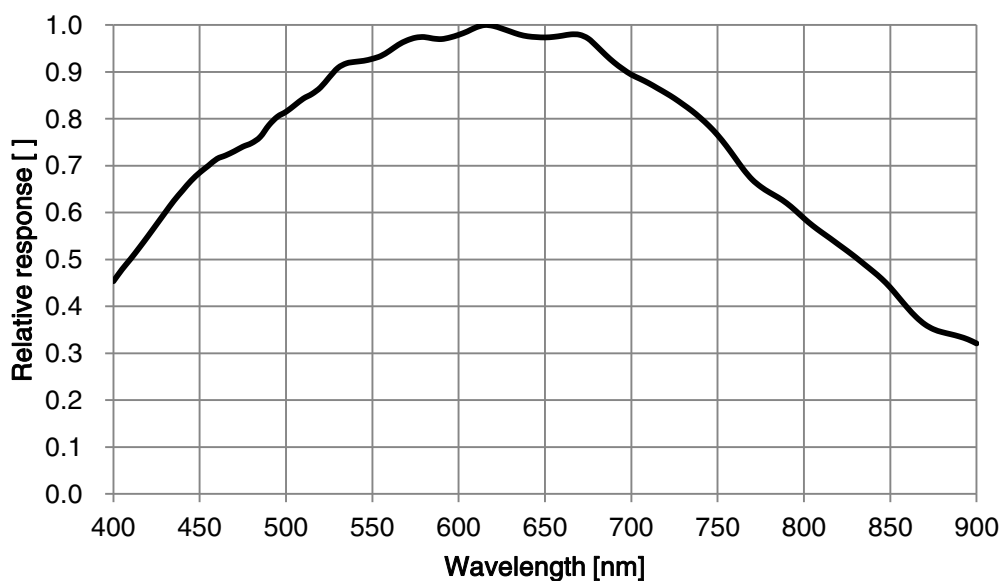
Figure 4-19 MER2-503-36U3M POL sensor spectral response
