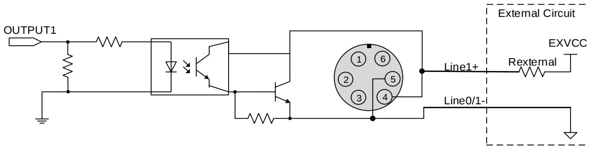
Figure 7-9 Opto-isolated output circuit (MER2-6P/ME2S)
