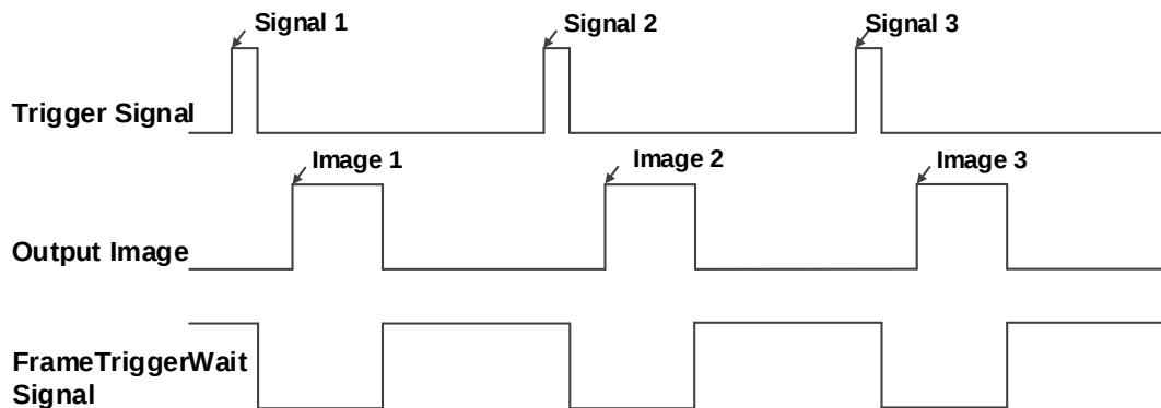
Figure 8-11 "FrameTriggerWait" signal schematic diagram
