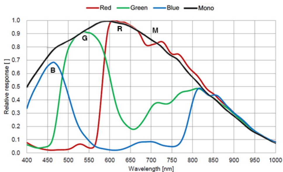
Figure 4-25 MER2-041-608U3M/C(-L)-HS sensor spectral response
