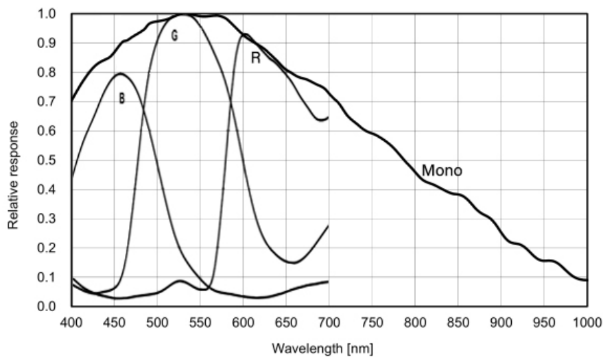
Figure 4-23 MER2-2000-19U3M/C(-L/-W90/-W90-S90) sensor spectral response
