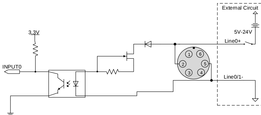
Figure 7-2 Opto-isolated input circuit (MER2-6P/ME2S)
