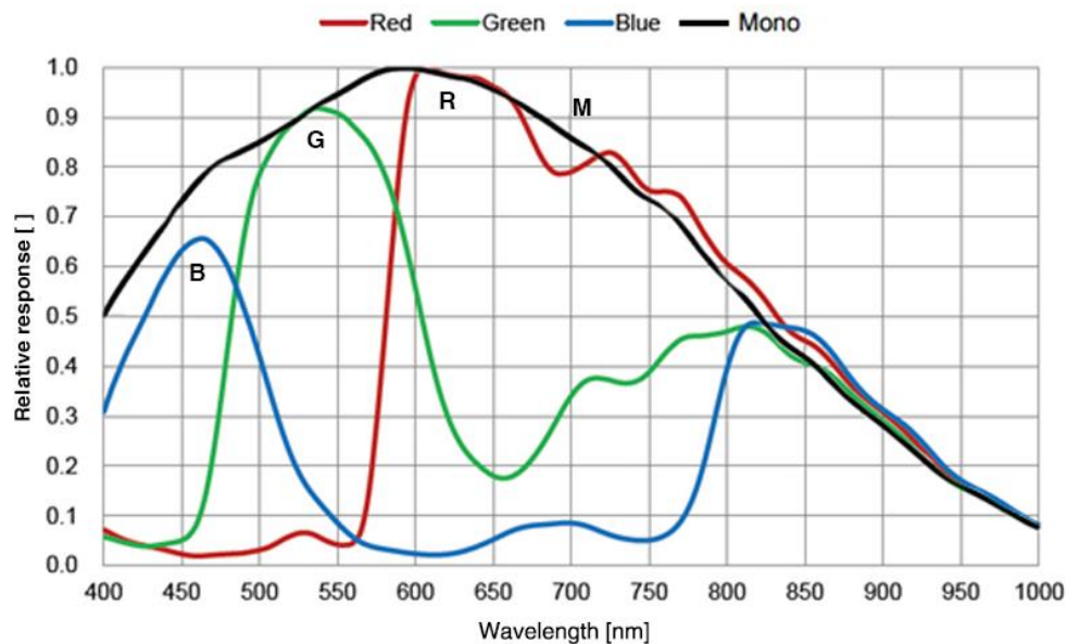
Figure 4-26 MER2-160-249U3M/C(-L)-HS sensor spectral response
