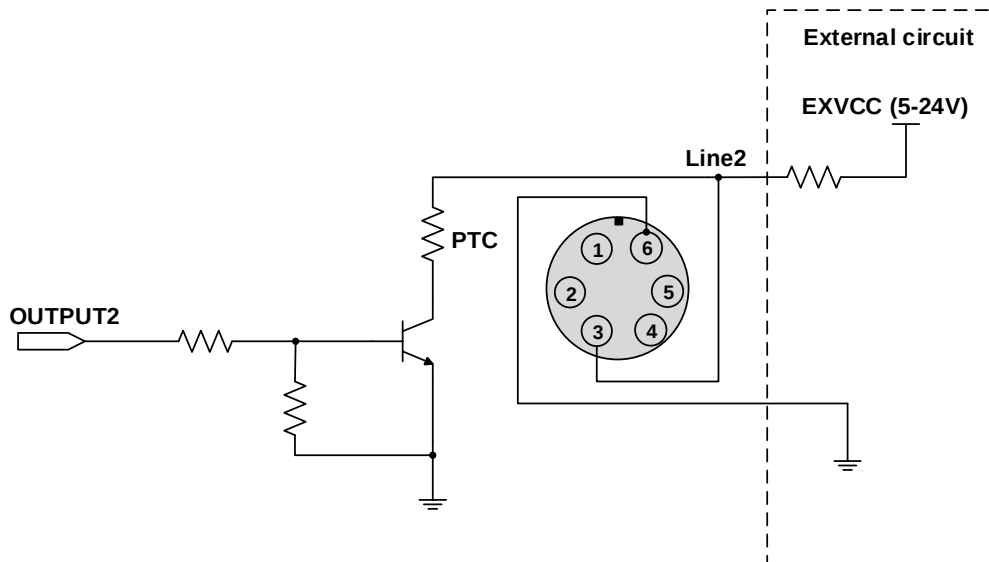
Figure 7-26 Internal equivalent circuit of camera when Line2 is configured as output (MER2-6P/ME2S)
