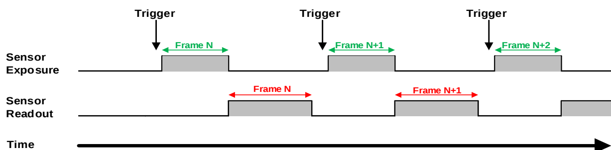
Figure 8-25 The trigger acquisition exposure sequence diagram in non-overlapping exposure mode
