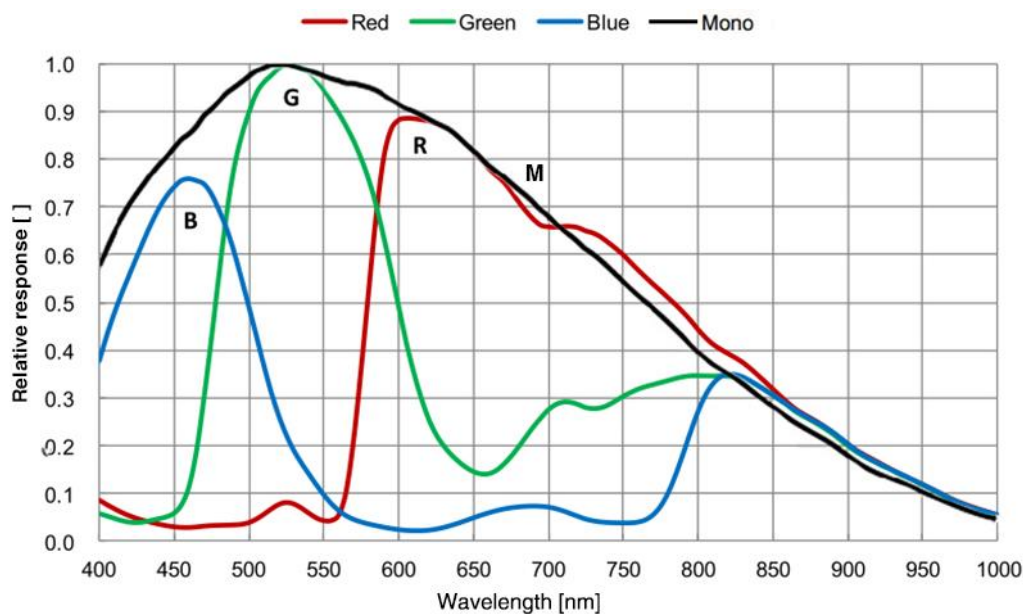
Figure 4-8 MER2-231-41U3M/C(-L) sensor spectral response
