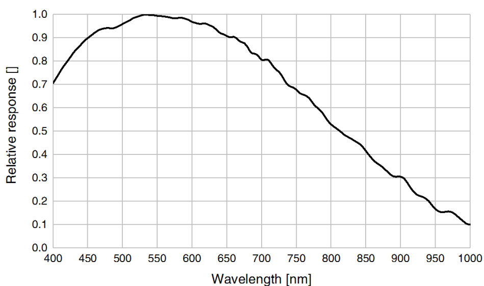
Figure 4-37 ME2S-2560-15U3M sensor spectral response
