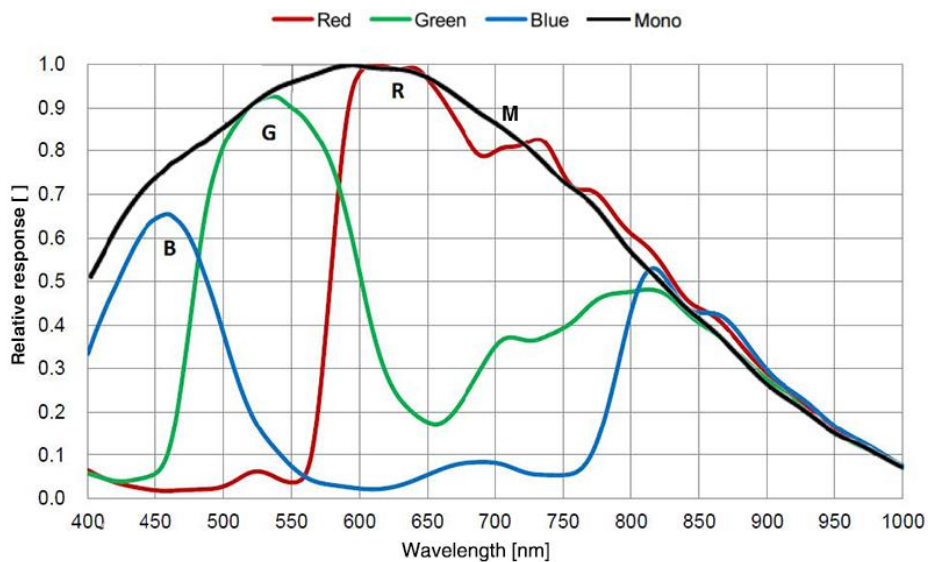
Figure 4-12 MER2-302-56U3M/C(-L) sensor spectral response
