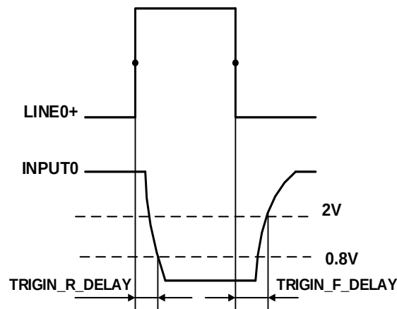
Figure 7-7 Parameter of opto-isolated input circuit
