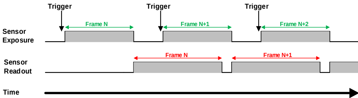
Figure 8-27 The trigger acquisition exposure sequence diagram in overlapping exposure mode
