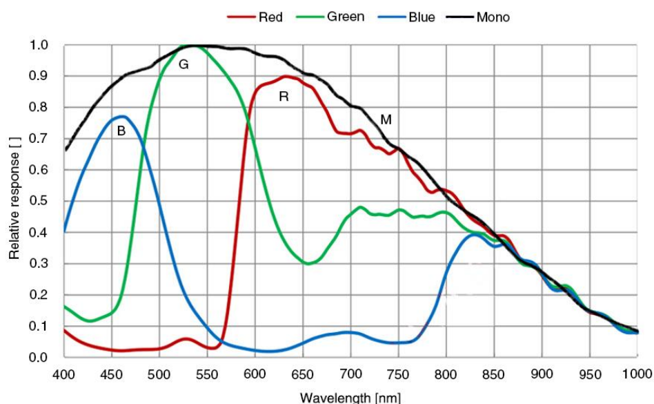
Figure 4-35 ME2S-2020-19U3M/C sensor spectral response
