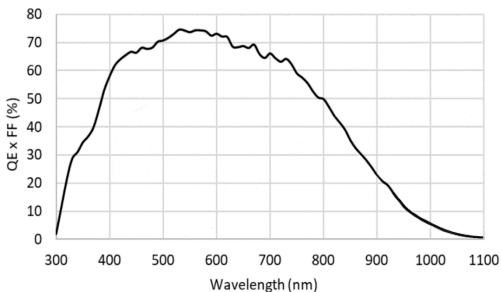
Figure 4-3 MER2-060-642U3M(-L) sensor spectral response
