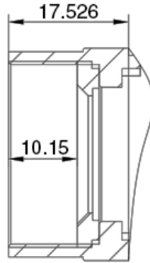
Figure 5-14 C-mount optical interface of ME2S
