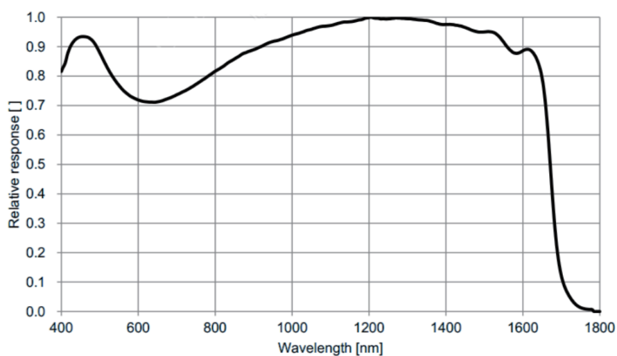
Figure 4-40 ME2S-138-232U3M-SWIR sensor spectral response
