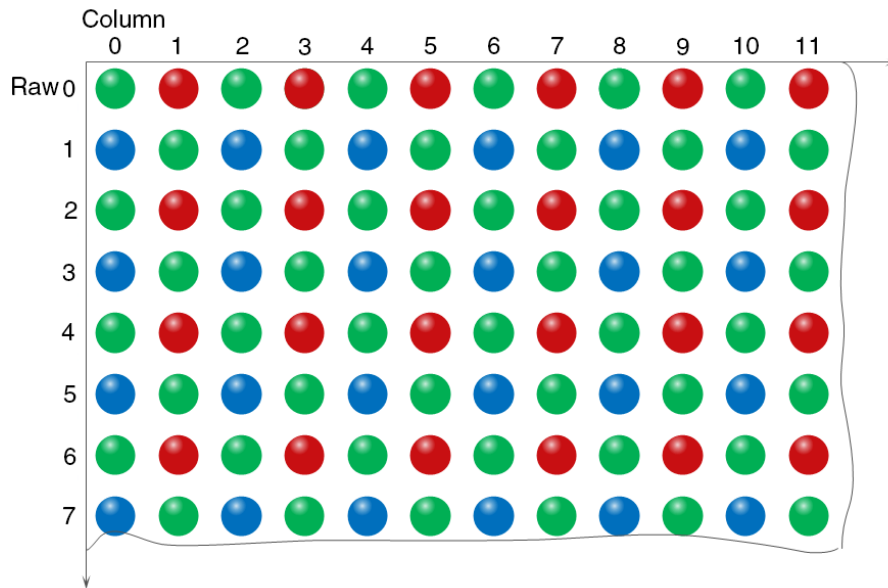
Figure 8-40 BayerGR8 pixel format
