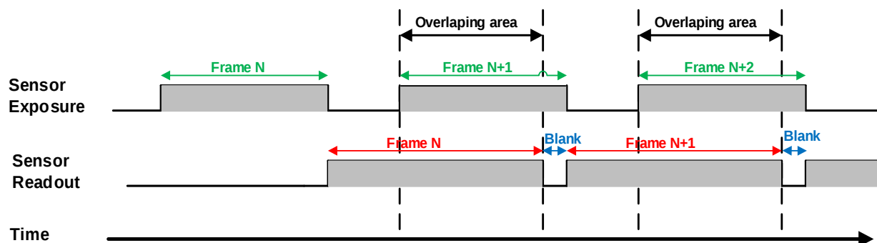
Figure 8-26 The exposure sequence diagram in overlapping exposure mode
