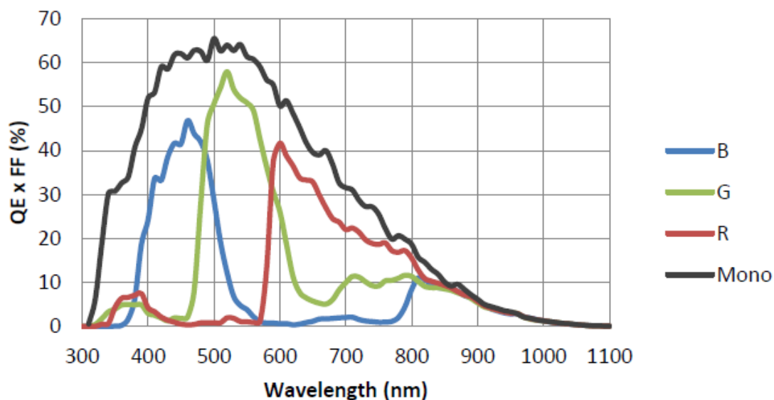
Figure 4-45 ME2P-900-43U3M/C sensor spectral response
