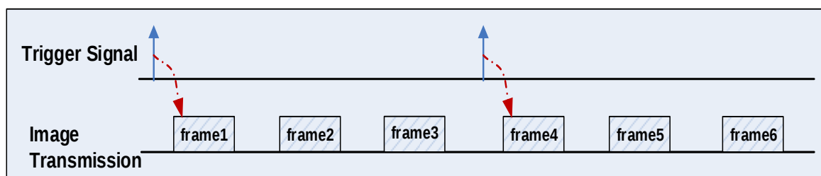
Figure 8-20 FrameBurstStart trigger
