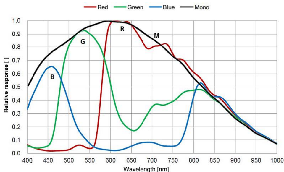
Figure 4-14 MER2-304-56U3M/C(-L) sensor spectral response
