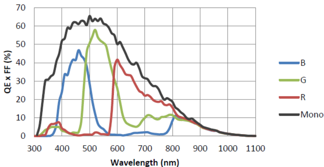
Figure 4-32 ME2S-560-70U3M/C sensor spectral response
