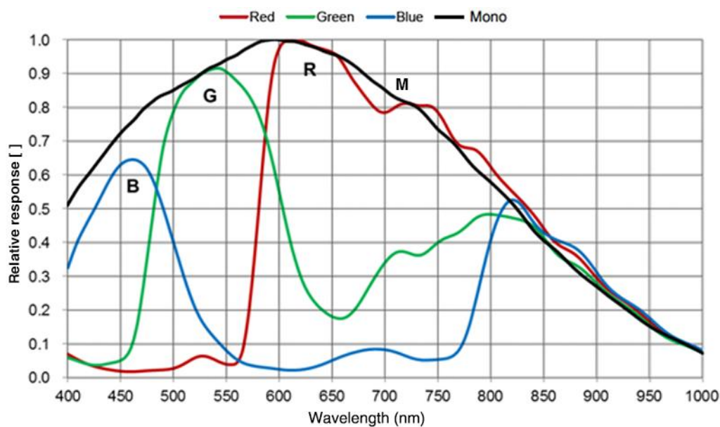
Figure 4-44 ME2P-883-42U3M/C sensor spectral response
