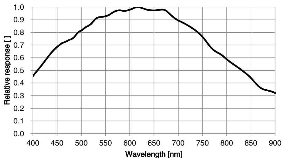
Figure 4-29 MER2-502-79U3M-HS POL sensor spectral response
