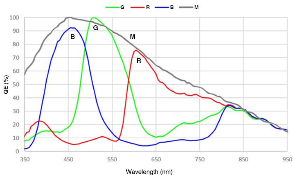
Figure 4-5 MER2-135-208U3M/C(-L) sensor spectral response
