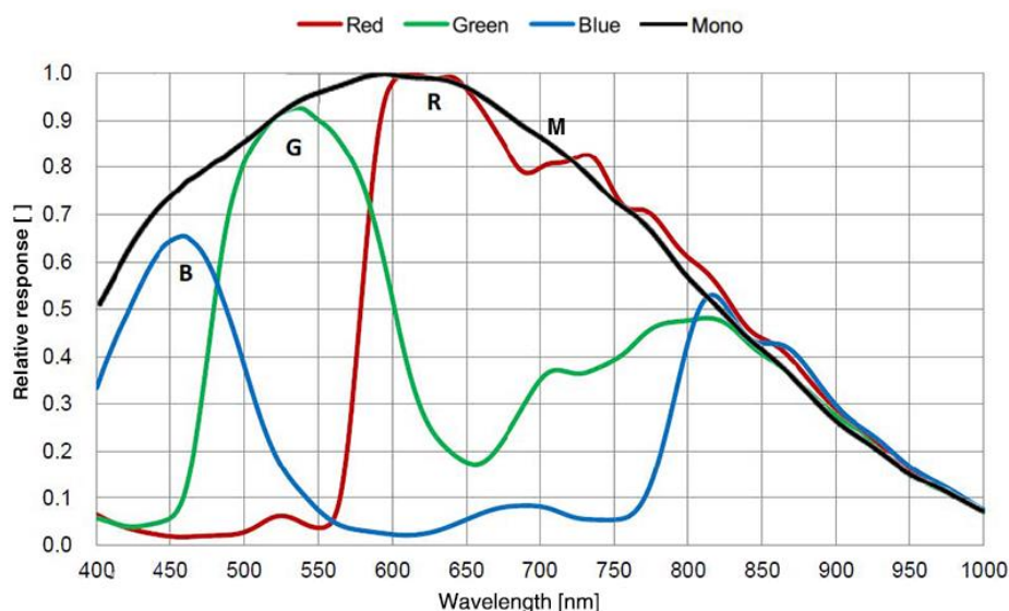
Figure 4-28 MER2-502-79U3M/C(-L)-HS sensor spectral response
