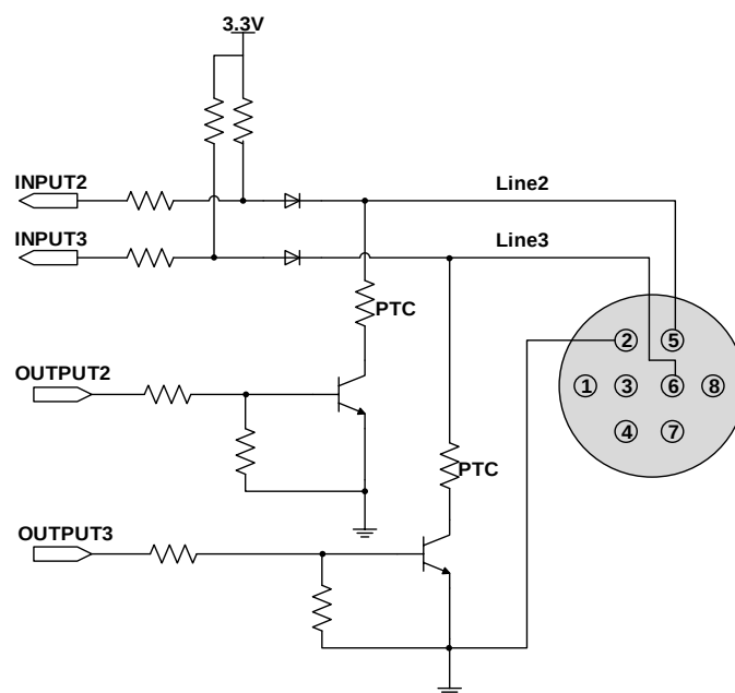
Figure 7-11 Line2/3 (bidirectional) circuit (MER2/ME2P)
