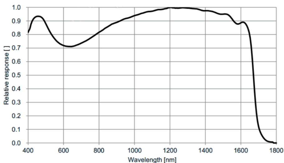
Figure 4-39 ME2S-138-136U3M-SWIR sensor spectral response
