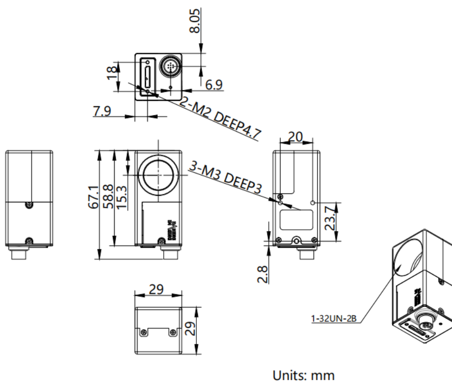
Figure 5-4 MER2-U3-W90-S90 mechanical dimensions
