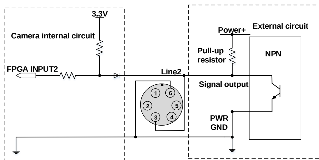
Figure 7-21 NPN photoelectric sensor connected to Line2 input circuit (MER2-6P/ME2S)
