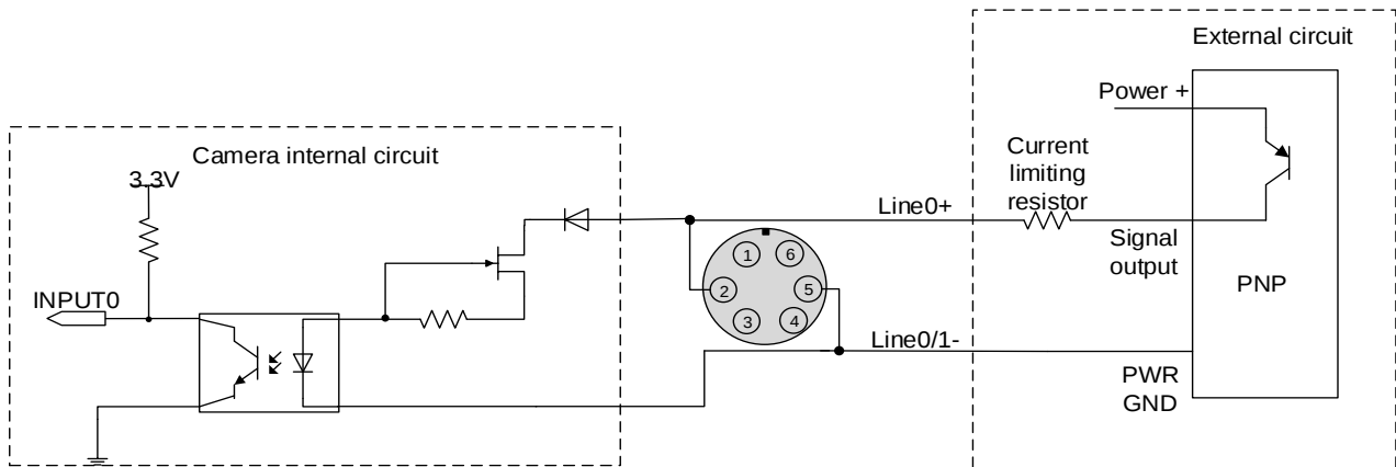
Figure 7-6 PNP photosensor connected to opto-isolated input circuit (MER2-6P/ME2S)
