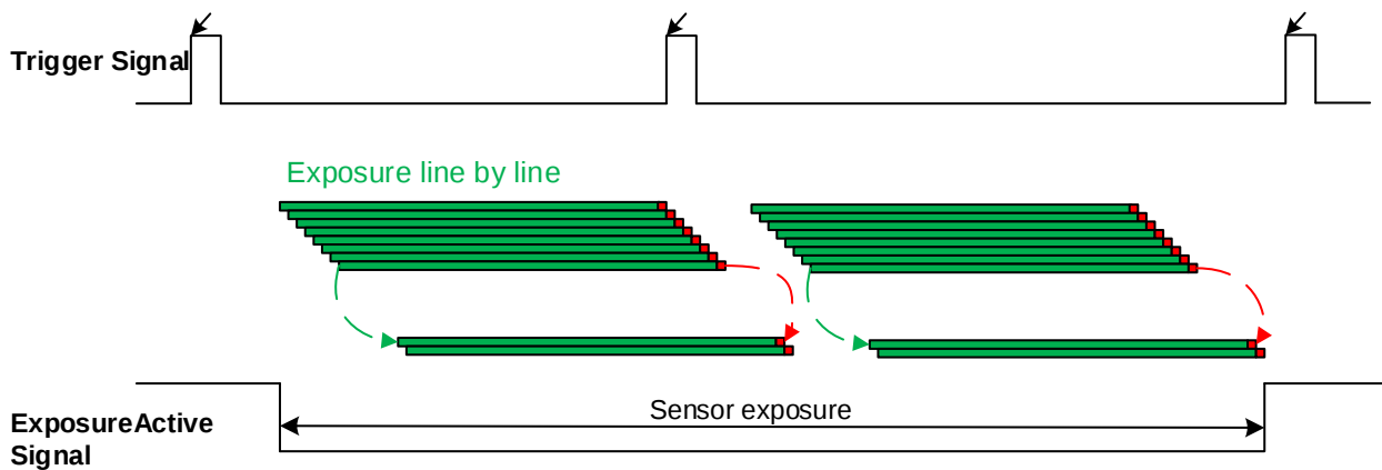
Figure 8-9 Electronic rolling shutter mode (overlapping exposure) "ExposureActive" signal schematic diagram
