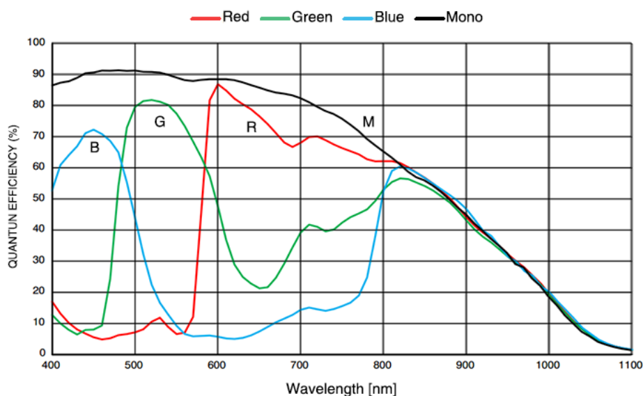
Figure 4-24 MER2-2002-20U3M/C(-L) sensor spectral response
