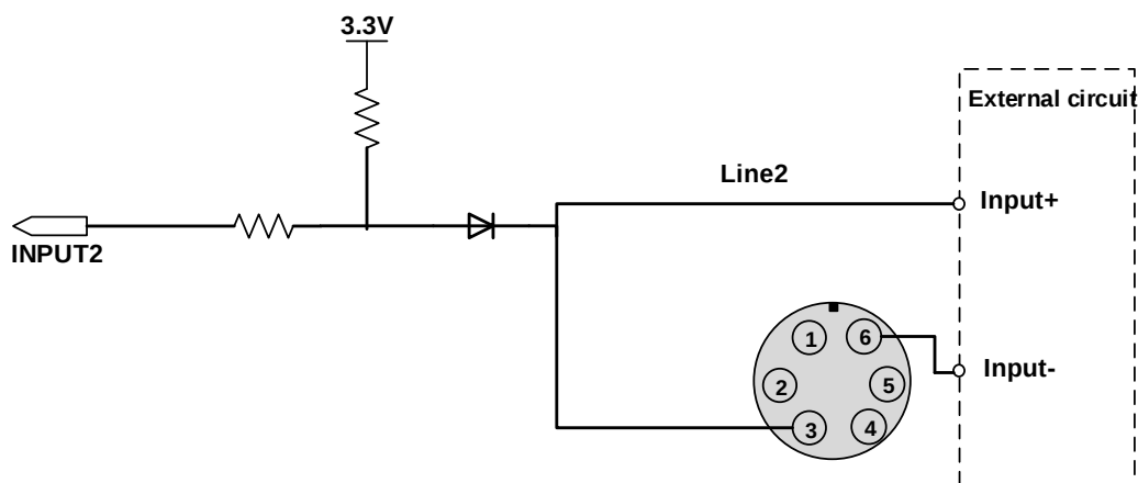
Figure 7-16 Internal equivalent circuit of camera when Line2 is configured as input (MER2-6P/ME2S)
