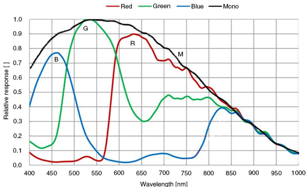
Figure 4-34 ME2S-1610-24U3M/C sensor spectral response
