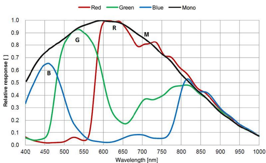
Figure 4-15 MER2-501-79U3M/C(-L) sensor spectral response
