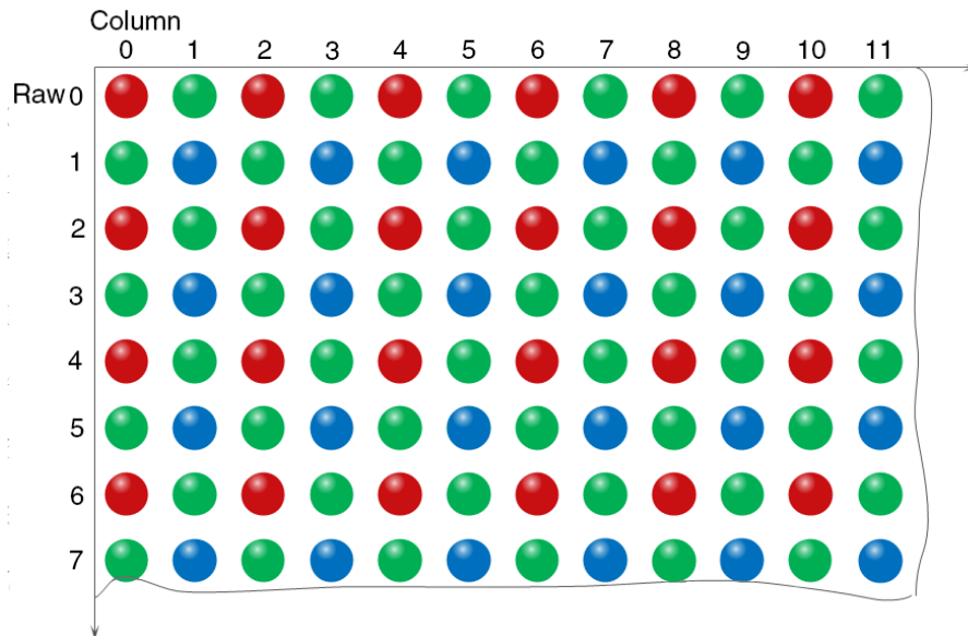
Figure 8-39 BayerRG8 pixel format
