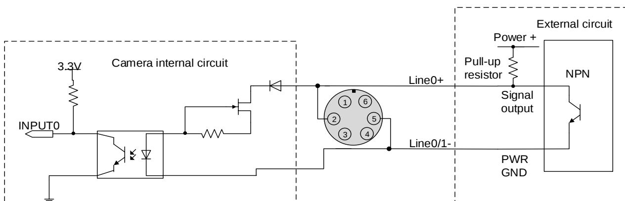
Figure 7-5 NPN photosensor connected to opto-isolated input circuit (MER2-6P/ME2S)
