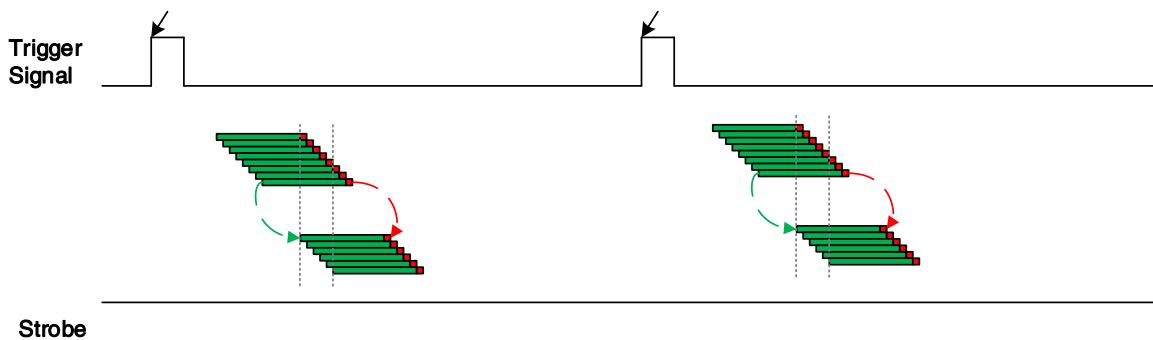
Figure 8-6 Strobe signal schematic diagram (all lines have no common exposure time in electronic rolling shutter)
