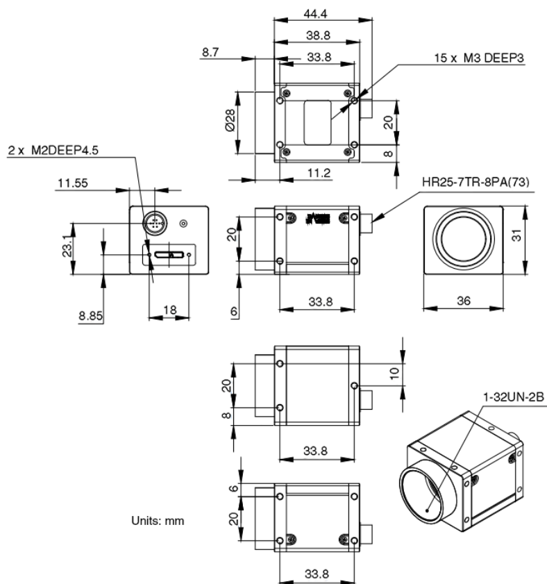
Figure 5-9 ME2P-U3 mechanical dimensions
