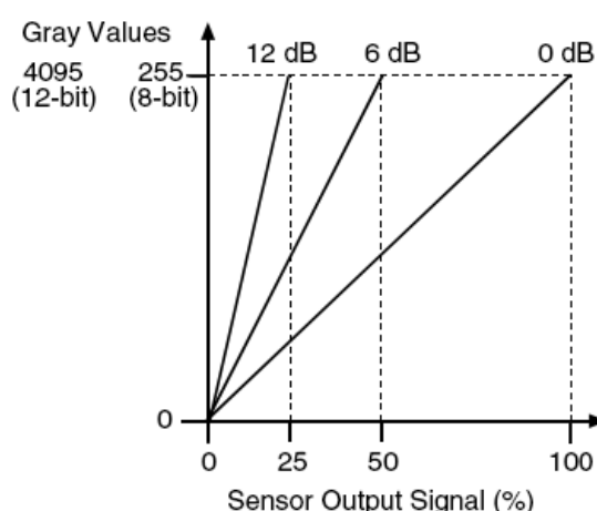
Figure 8-37 The cameras response curve
