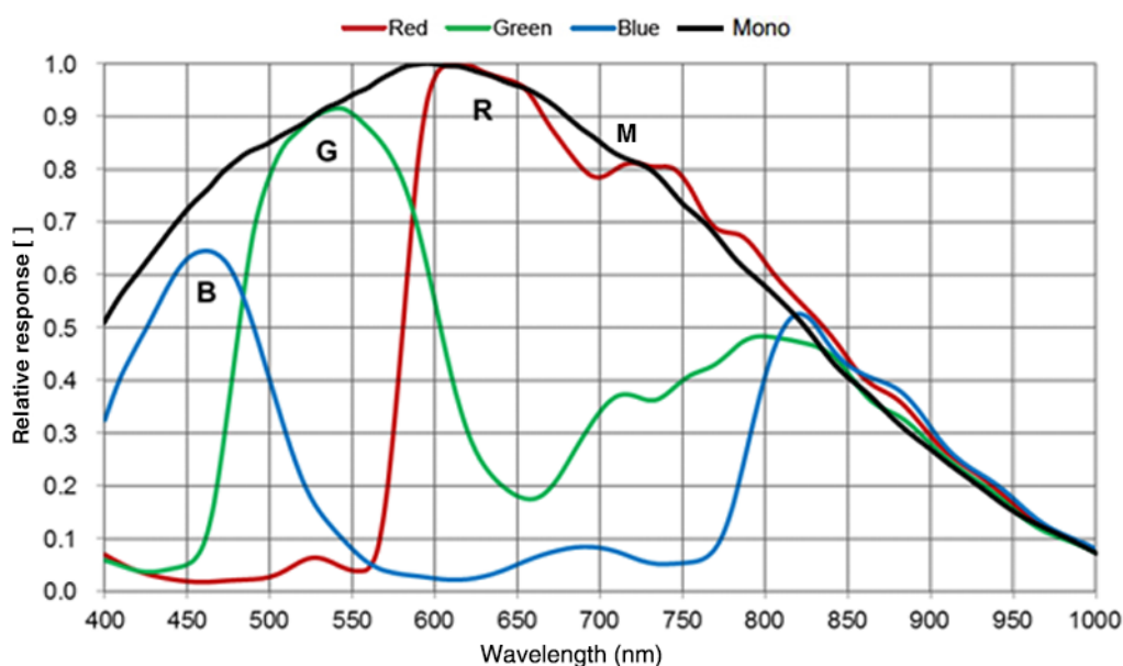
Figure 4-55 ME2P-1230-30U3M/C-HS sensor spectral response
