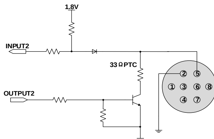
Figure 7-12 Line2 (bidirectional) circuit (ME2L)
