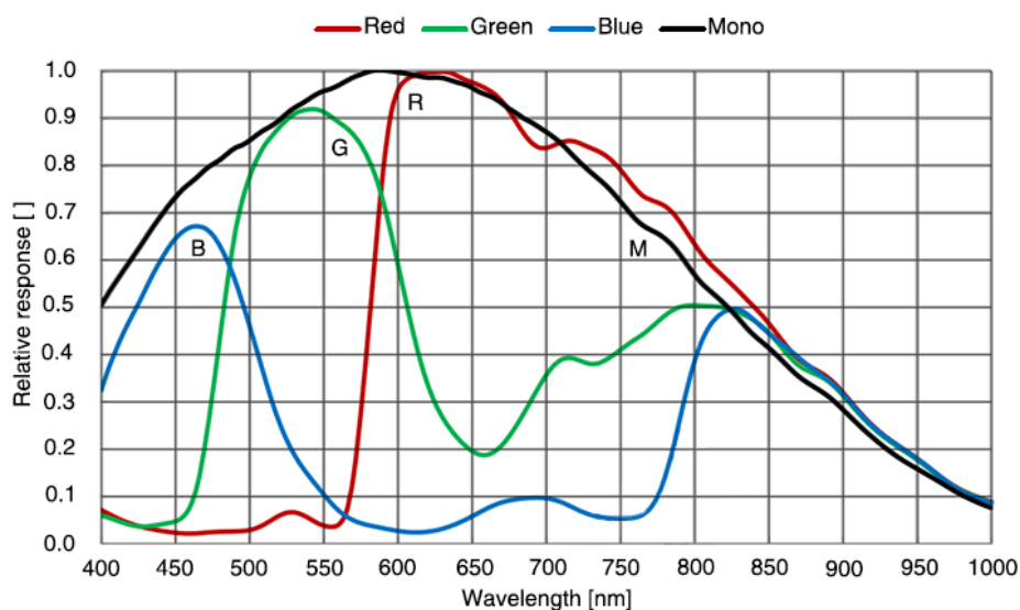
Figure 4-41 ME2P-170-210U3M/C sensor spectral response
