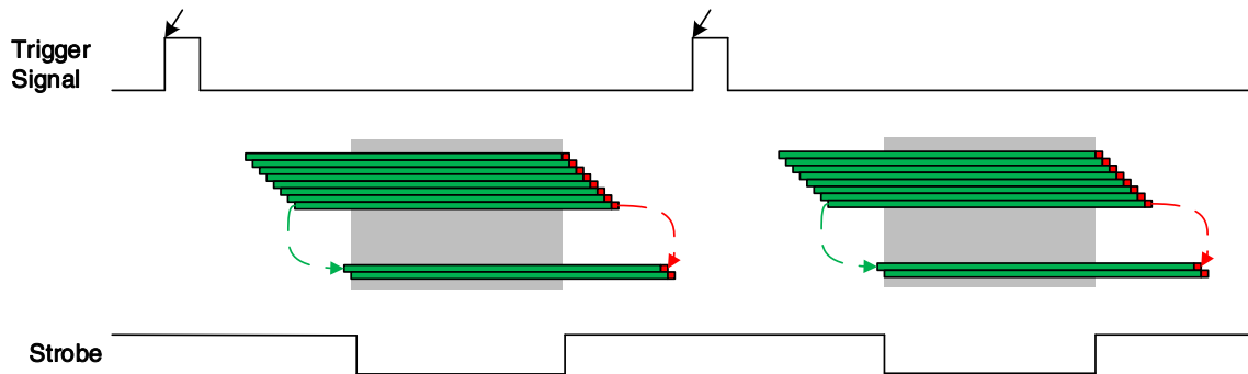
Figure 8-5 Strobe signal schematic diagram (all lines have common exposure time in electronic rolling shutter)
