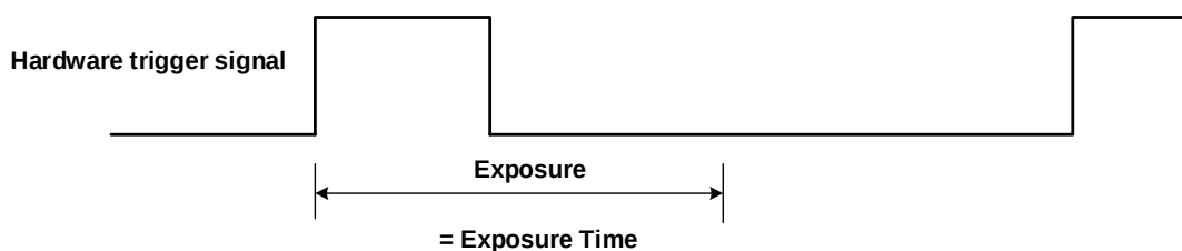
Figure 8-28 The sequence diagram in rising edge trigger of Timed exposure mode
