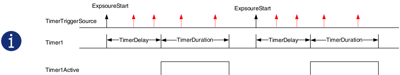
Figure 8-67 The relationship of Timer1Active and ExposureStart signal
