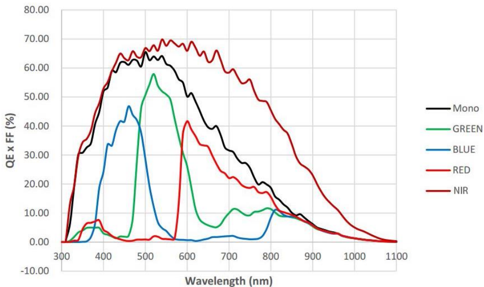
Figure 4-50 ME2P-2621-15U3M/C \ ME2P-2622-15U3M/C sensor spectral response
