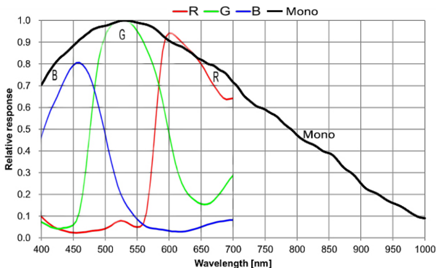
Figure 4-21 MER2-630-60U3M/C(-L/-W90/-W90-S90) sensor spectral response
