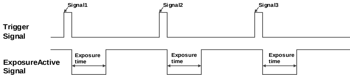
Figure 8-7 Global shutter mode "ExposureActive" signal schematic diagram
