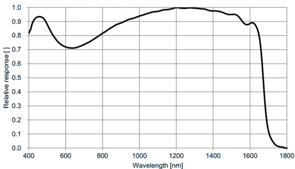
Figure 4-38 ME2S-033-262U3M-SWIR sensor spectral response
