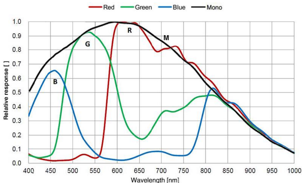
Figure 4-20 MER2-510-36U3M/C(-L) sensor spectral response
