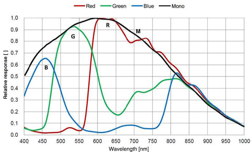
Figure 4-13 MER2-303-107U3M/C(-L) sensor spectral response
