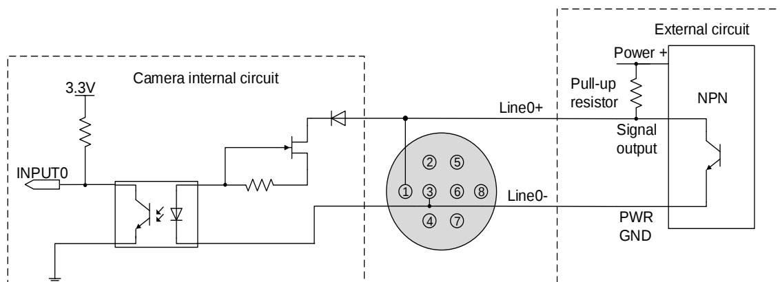
Figure 7-3 NPN photosensor connected to opto-isolated input circuit (MER2/ME2P/ME2L)
