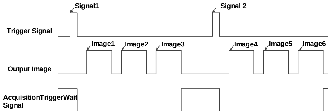
Figure 8-12 "AcquisitionTriggerWait" signal schematic diagram
