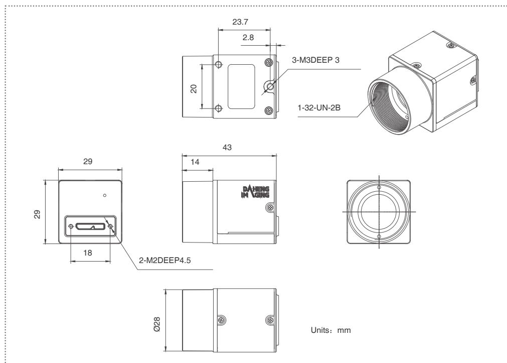
MER2-280-139U3M/C-L
