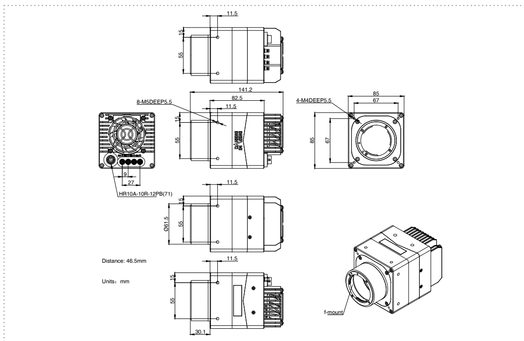
MARS-6501-31X2M/C-TF (F-mount)
