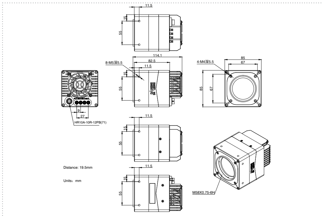
MARS-6501-31X2M/C-TF (M58-mount)
